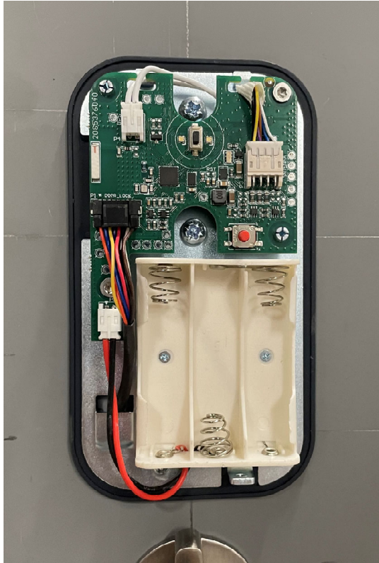
Photo of the Rear Mount Back with Batteries removed
