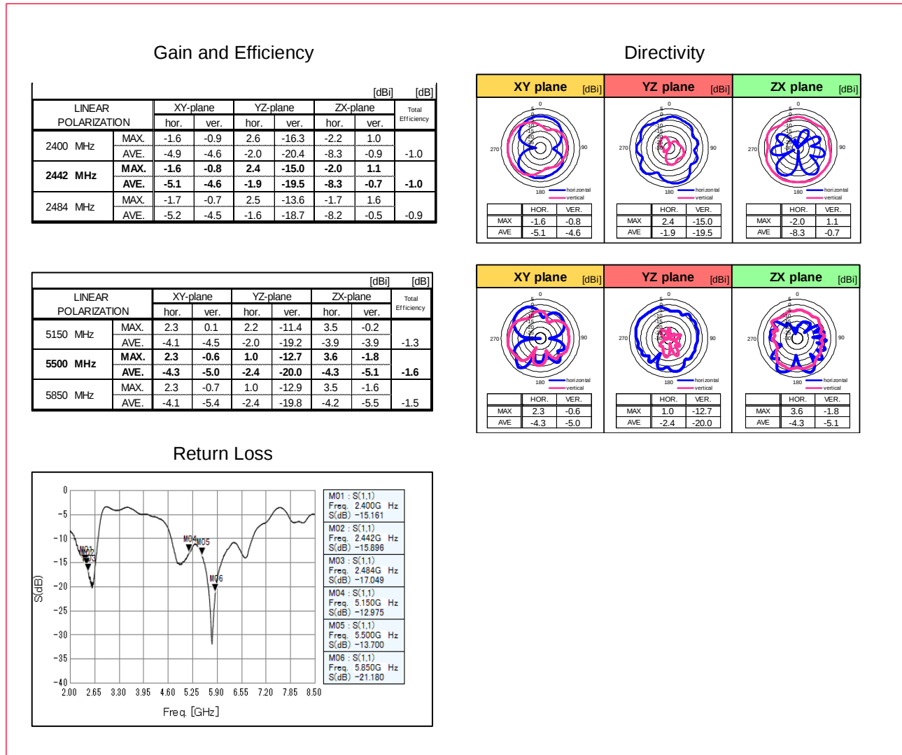
Figure 14: Trace Antenna Performance
