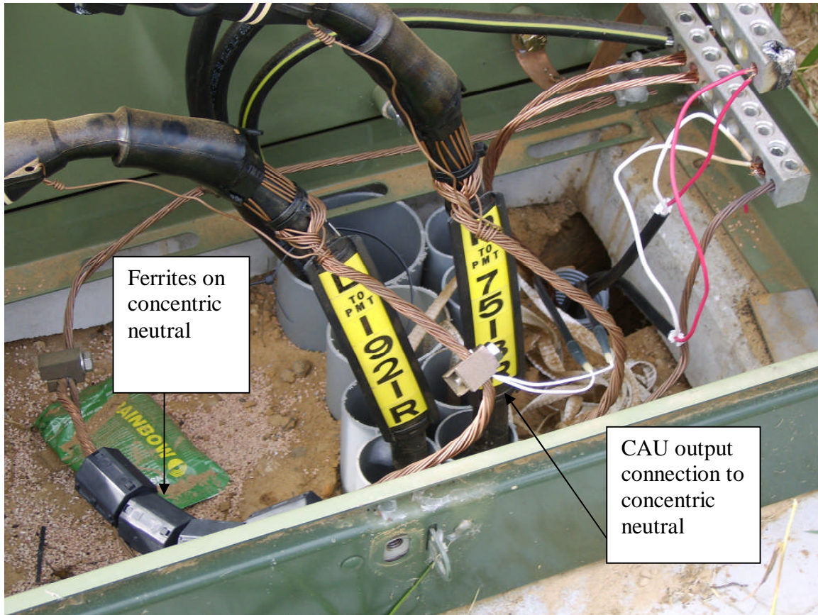
CAU padmount coupler connection
