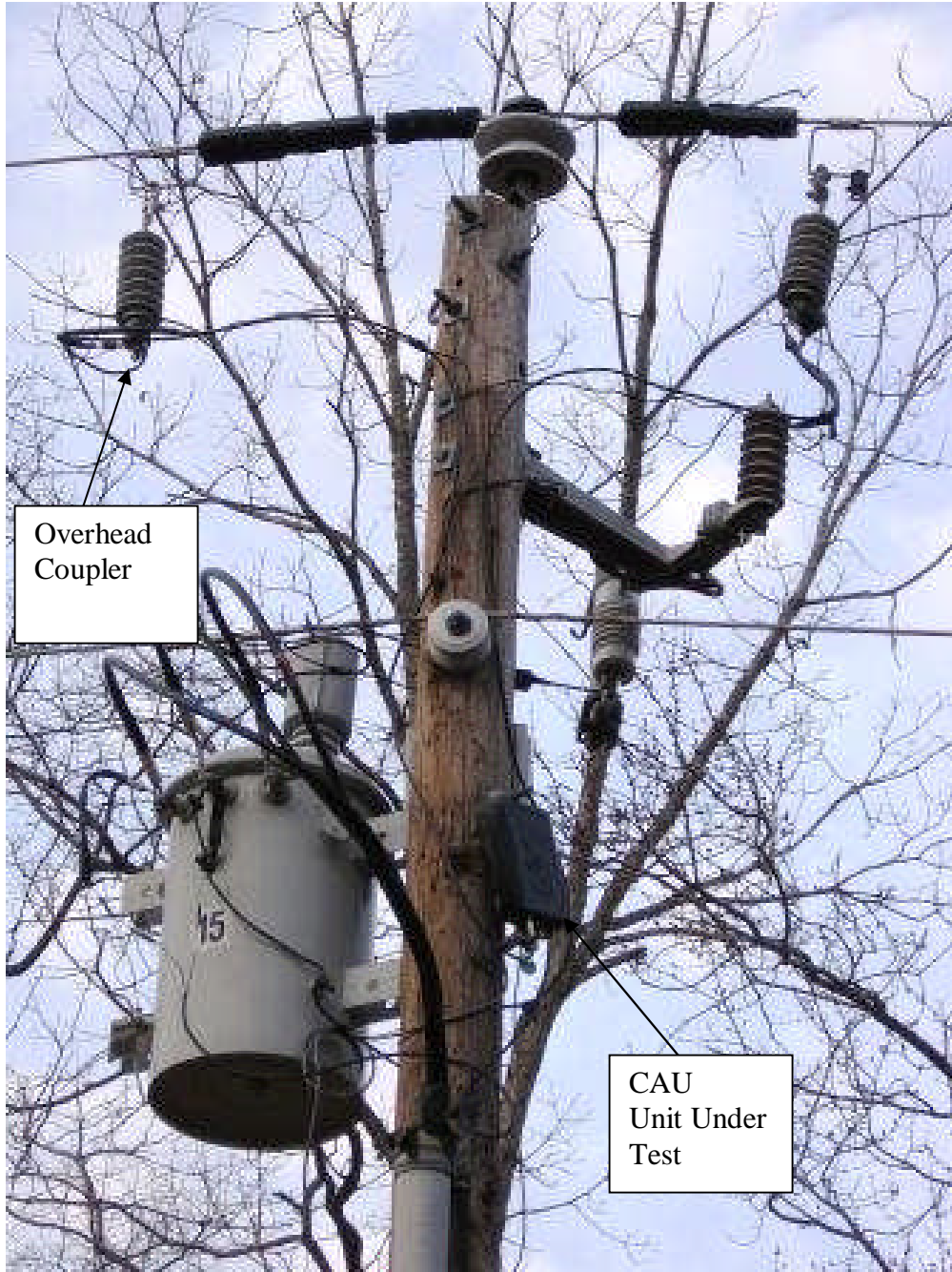
CAU overhead mounting
