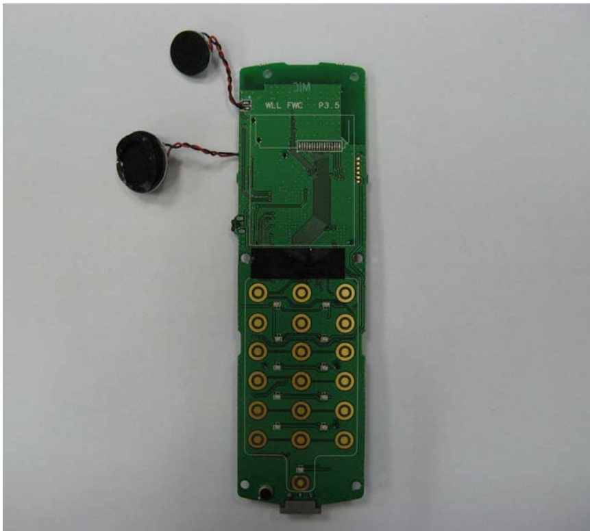
Picture2: Front view of PCB with screen removed
