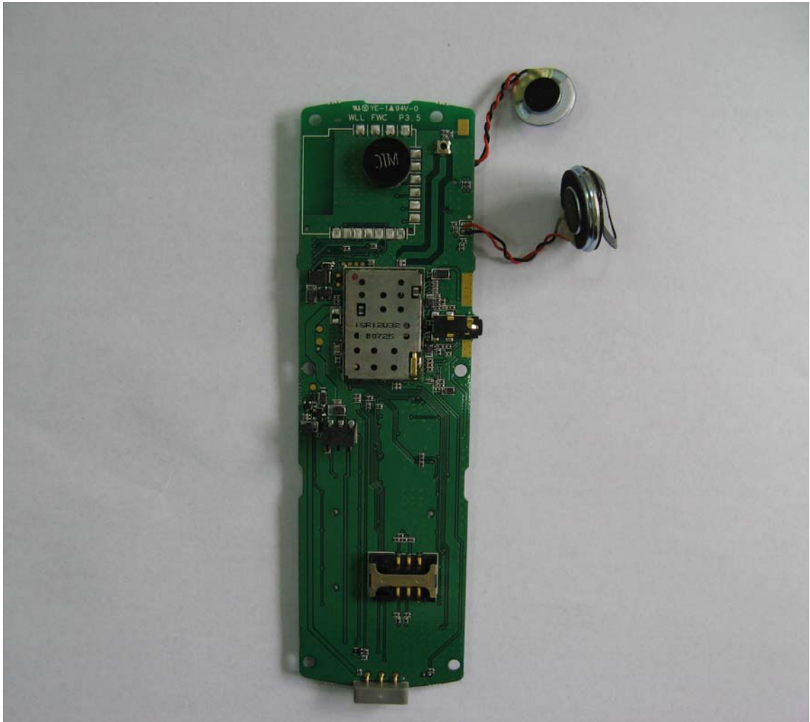
Picture3: Back view of PCB
