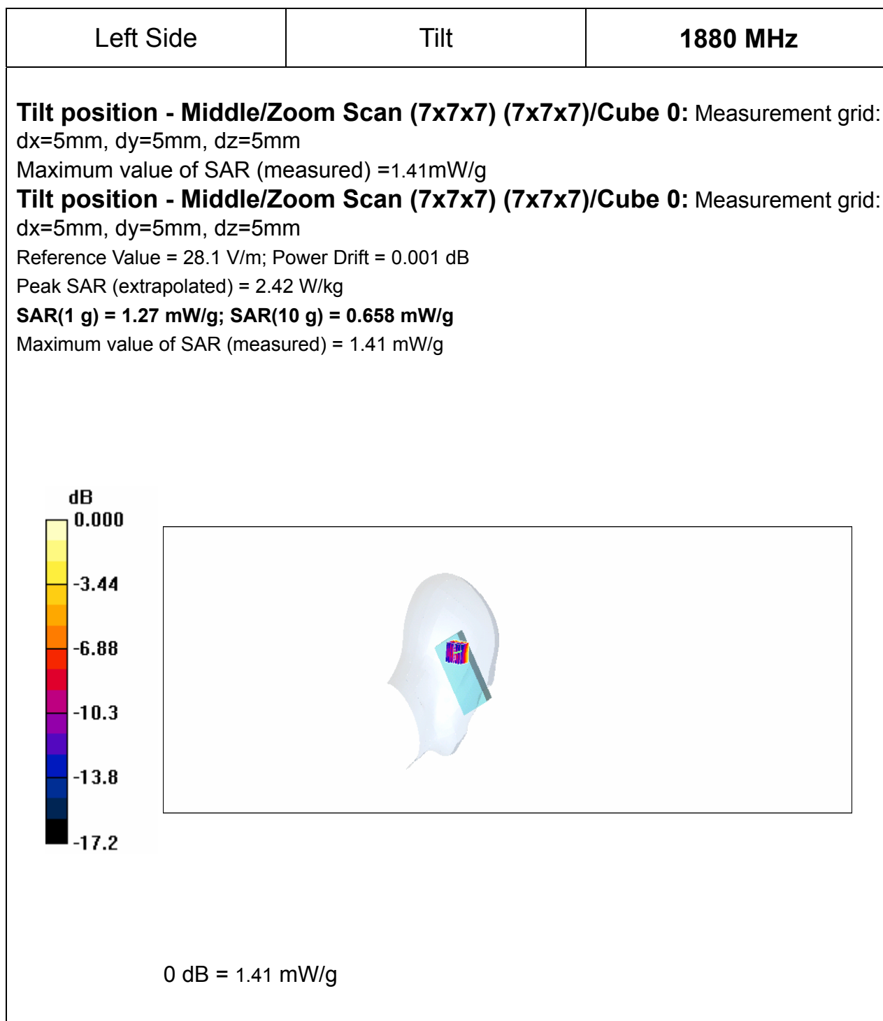
Fig26 SAR Test result
