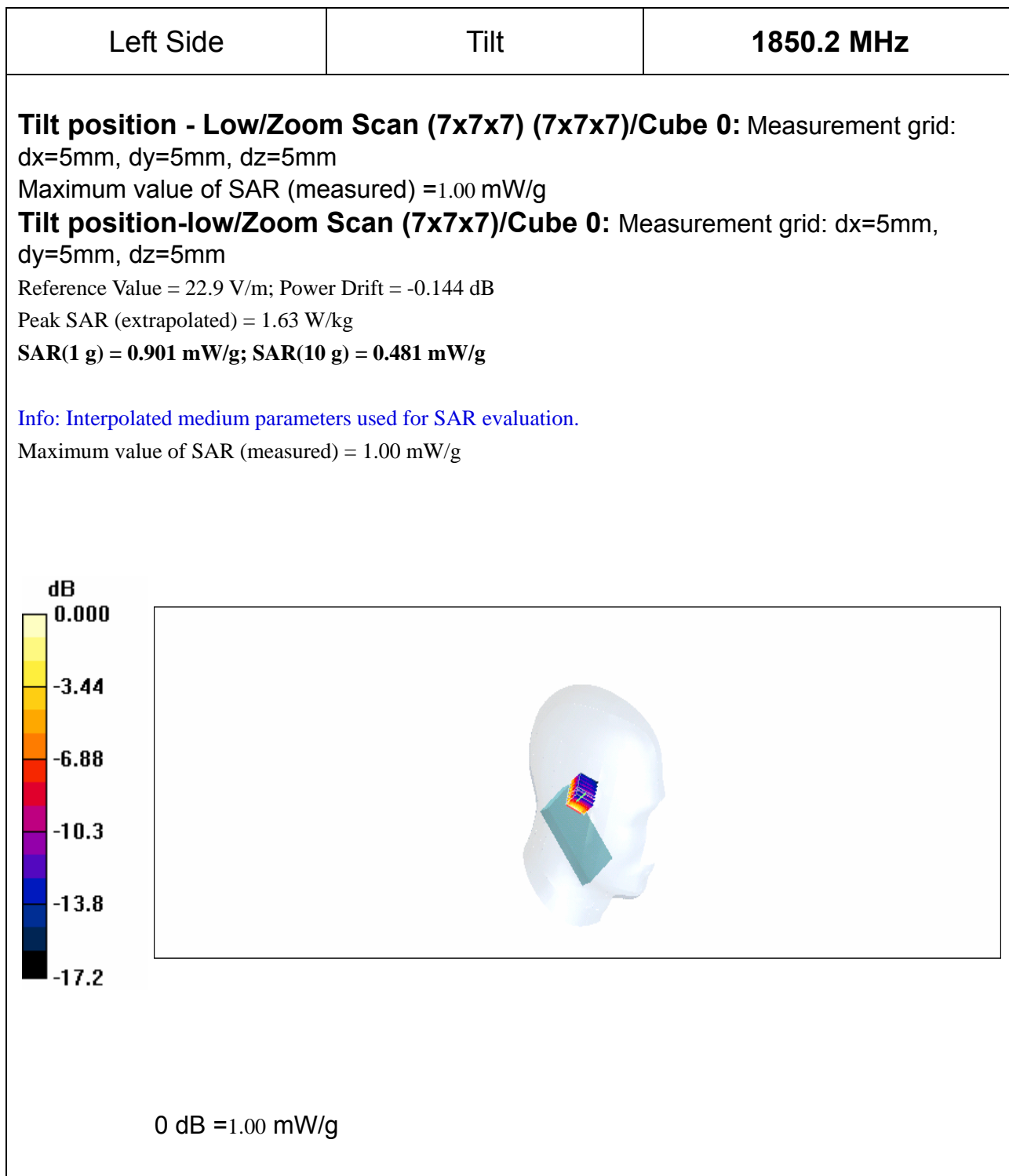
Fig25 SAR Test result
