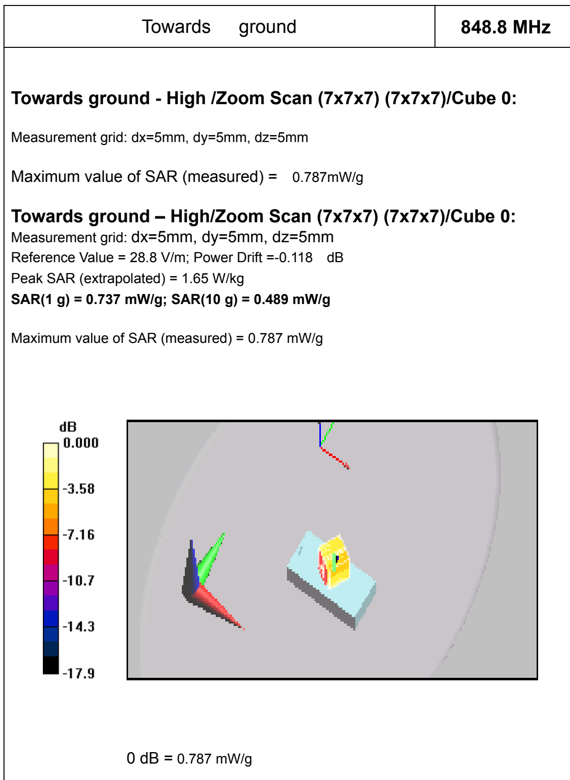
Fig30 SAR Test result
