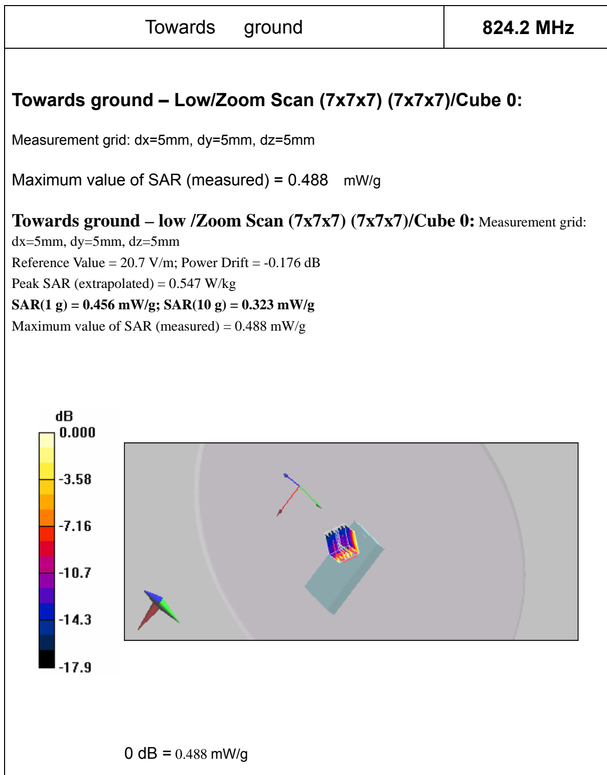
Fig31 SAR Test result
