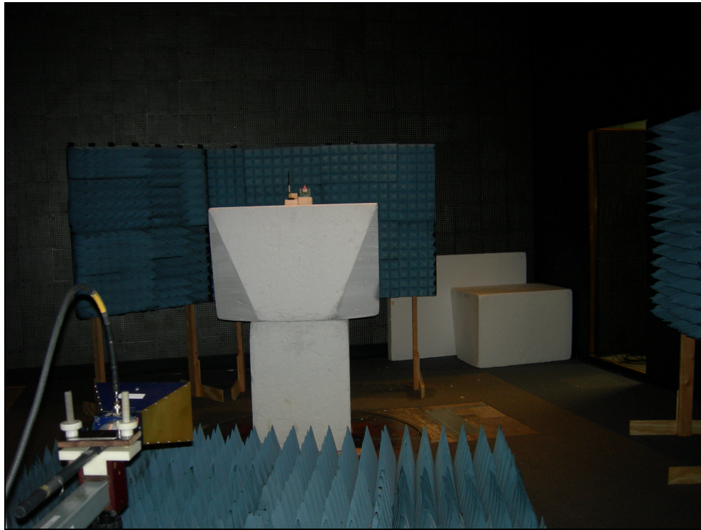
Figure 9: Radiated Emissions – U.FL – YPOS
