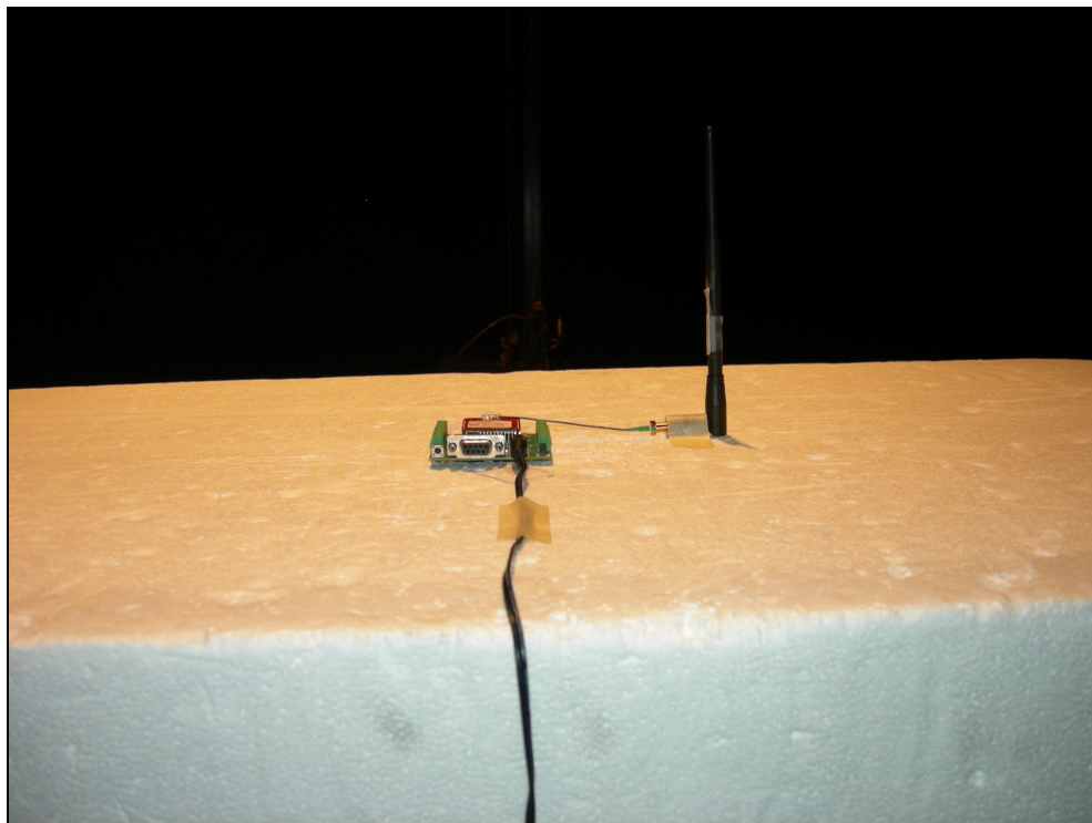
Figure 8: Radiated Emissions – U.FL – XPOS
