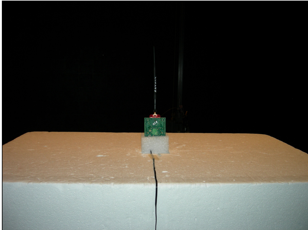
Figure 4: Radiated Emissions – SMA Port – YPOS
