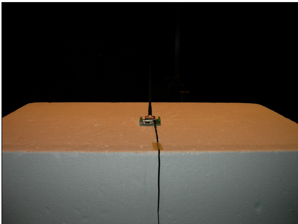
Figure 2: Radiated Emissions – SMA Port – XPOS
