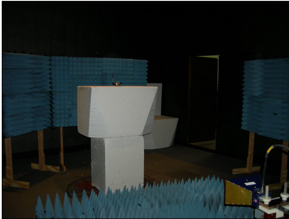
Figure 5: Radiated Emissions – SMA Port – ZPOS
