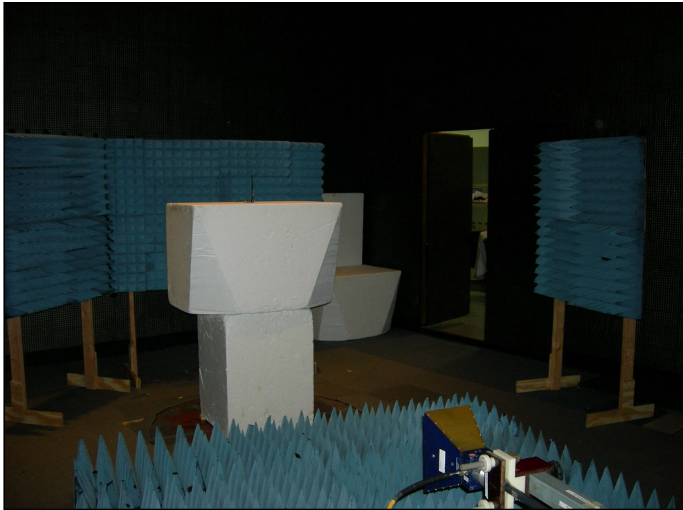
Figure 1: Radiated Emissions – SMA Port – XPOS
