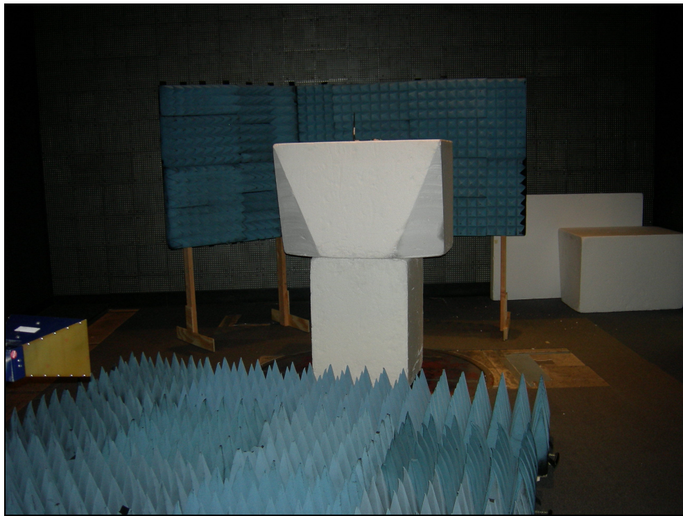
Figure 7: Radiated Emissions – U.FL – XPOS
