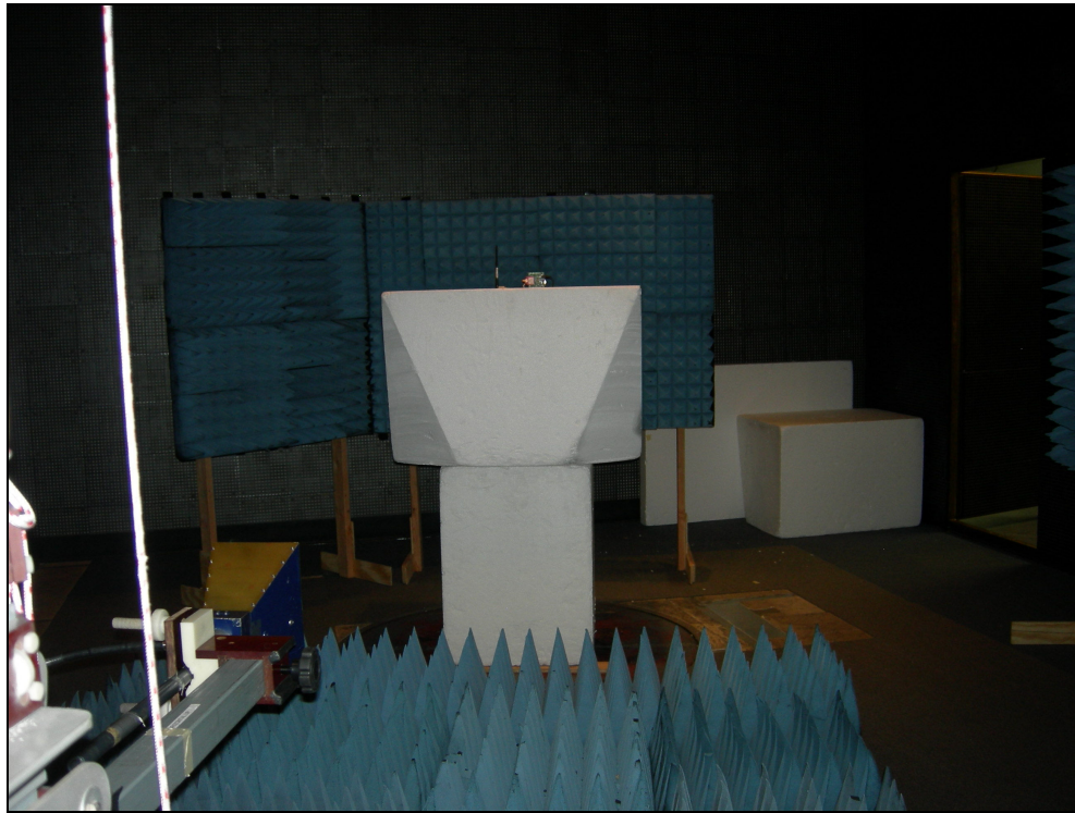
Figure 11: Radiated Emissions – U.FL – ZPOS
