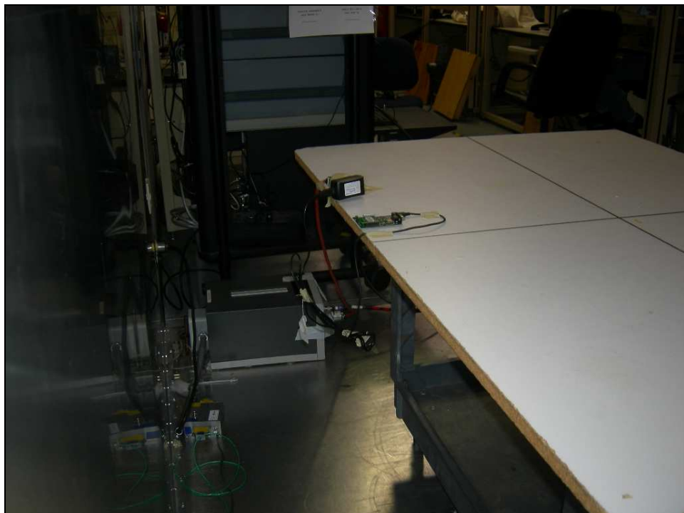
Figure 4: Conducted Emissions – Side View
