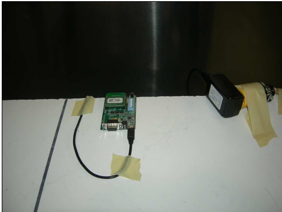
Figure 3: Conducted Emissions – Front View
