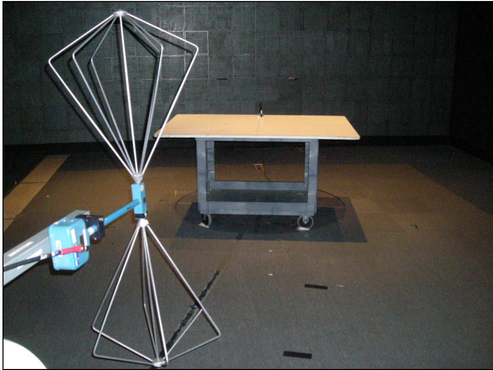
Figure 5: Radiated Emissions
