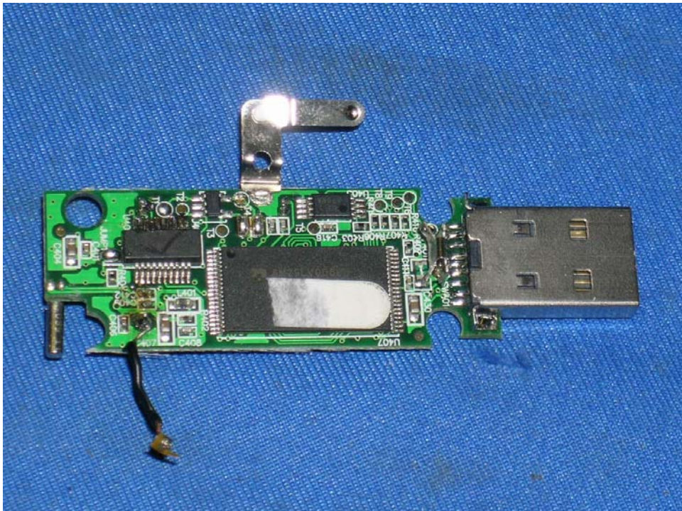
Keychain Remote Main PCB comp side
