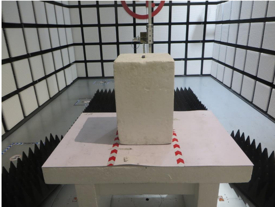
RADIATED RF MEASUREMENT SETUP (ABOVE 1 GHz) MEASUREMENT POSITION
