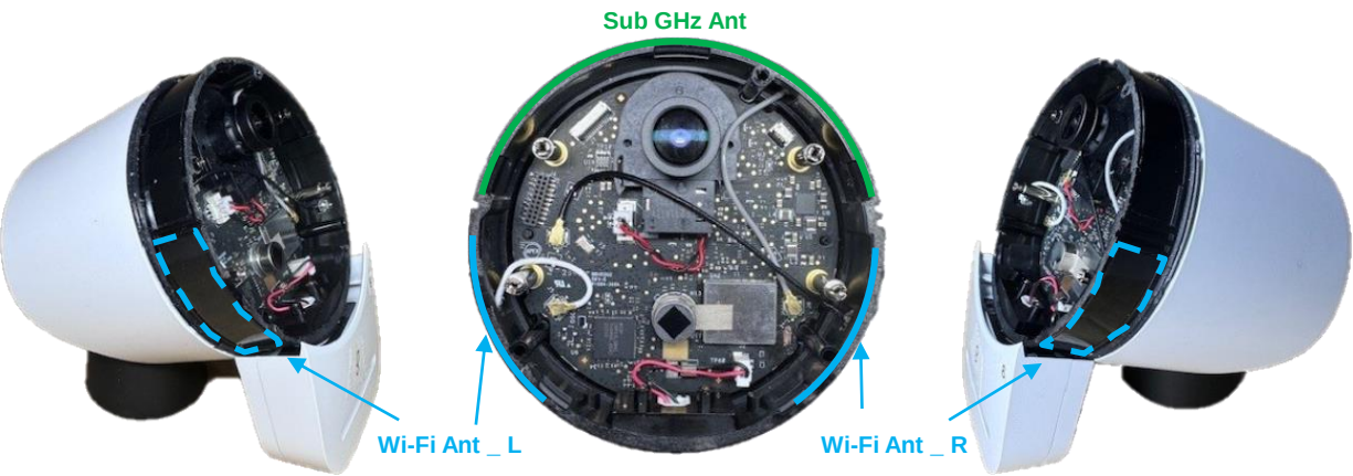
Left View
