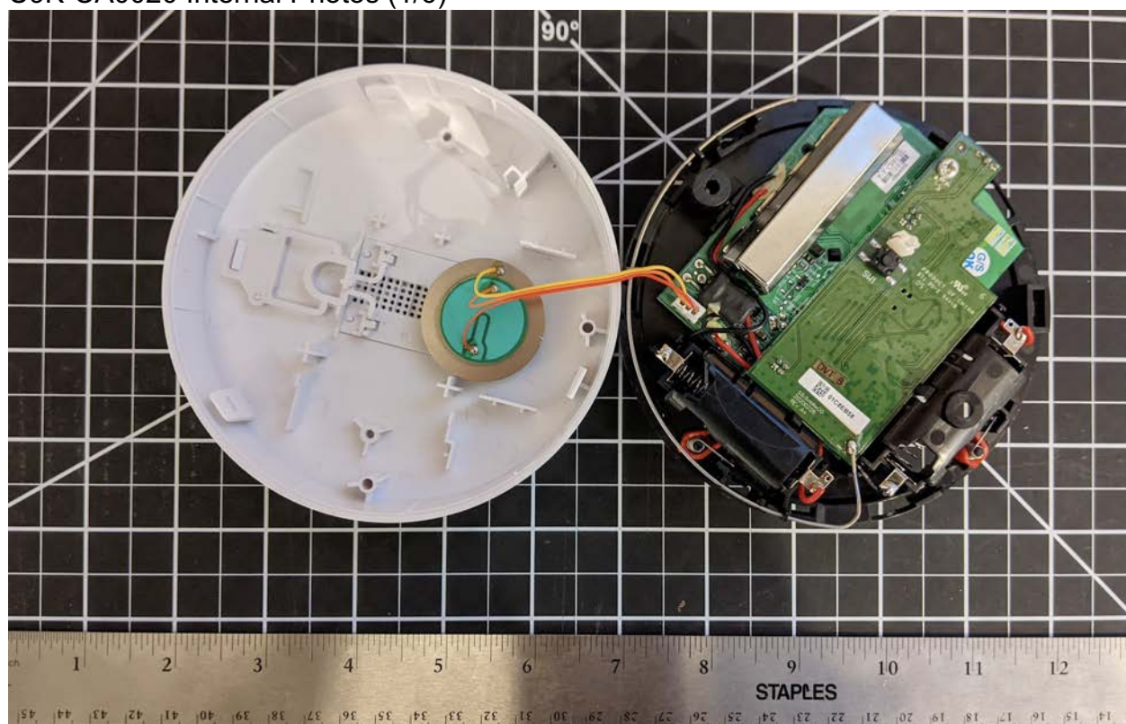
U9K-CA0020 Internal Photos (1/6)
