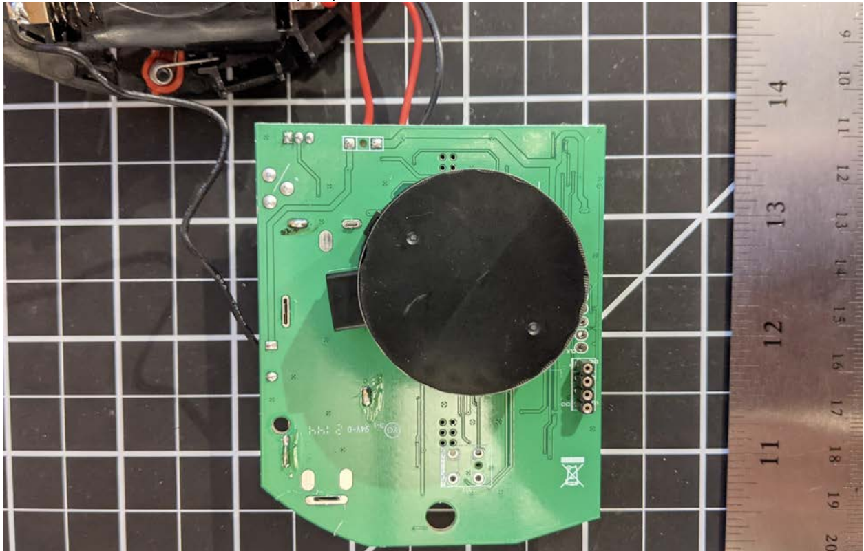
U9K-CA0020 Internal Photos (5/6)
