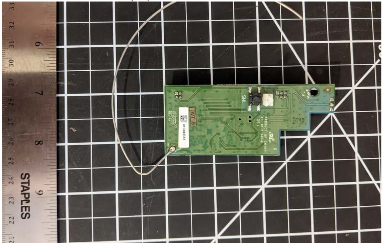
U9K-CA0020 Internal Photos (3/6)
