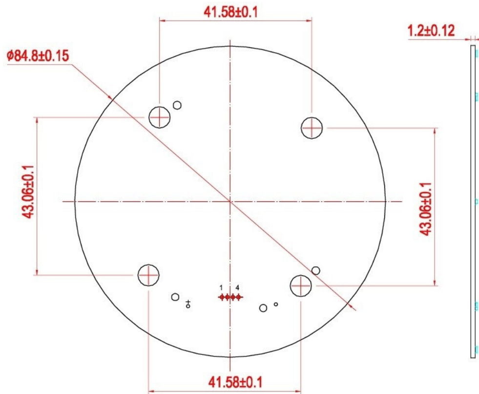
TOP VIEW
