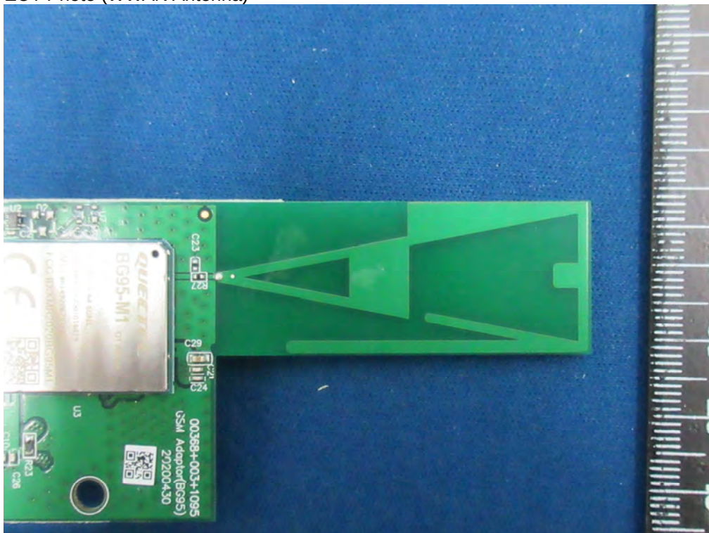
(14) EUT Photo (WWAN Antenna)
