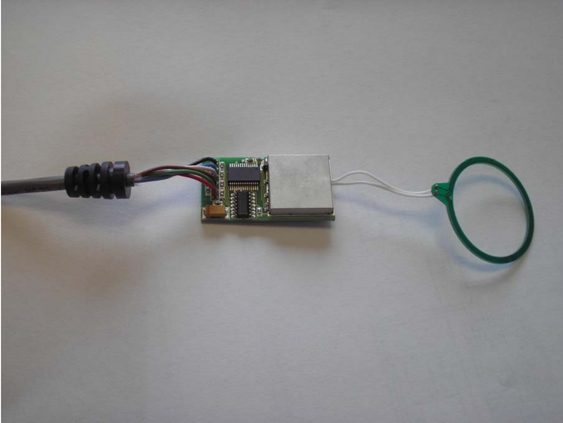
U9IUDC12-PM Circuit Board, Assembly
