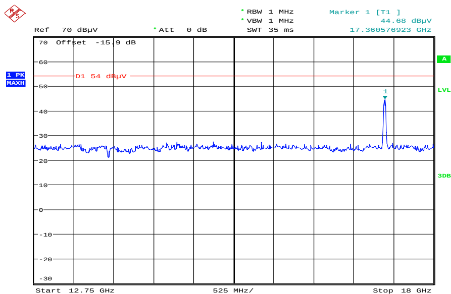
Plot 15: TX mode, mid channel – 5785 MHz, 12.75 GHz – 18 GHz, vertical & horizontal polarization
