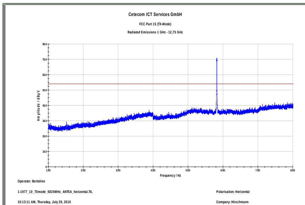
Plot 21: TX mode, high channel – 5825 MHz, 1 GHz – 8 GHz, horizontal polarization
