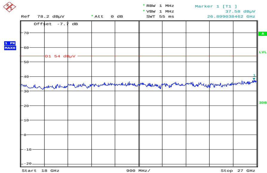
Plot 6: RX mode, 18 GHz – 27 GHz, vertical & horizontal polarization
