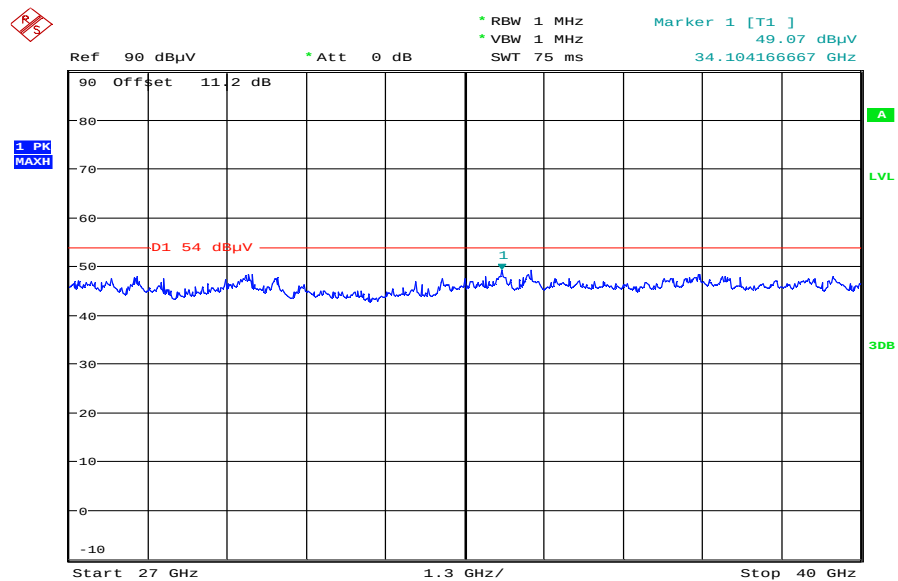
Plot 17: TX mode, mid channel – 5785 MHz, 27 GHz – 40 GHz, vertical & horizontal polarization
