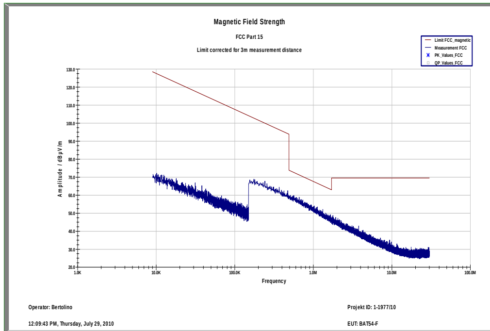
Plot 9: TX mode, mid channel – 5785 MHz, 9 kHz – 30 MHz, magnetic
