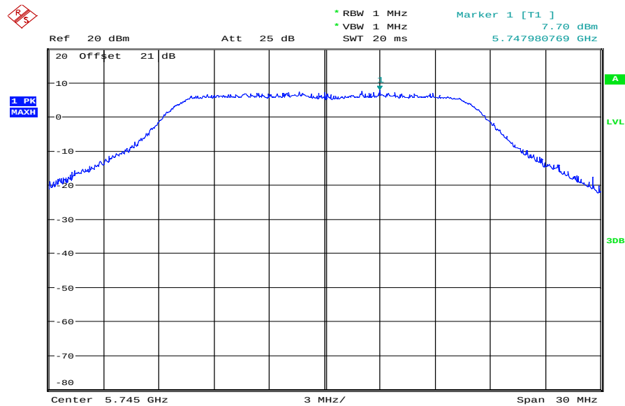
Plot 1: TX mode, low channel – 5745 MHz, power @ 1 MHz
