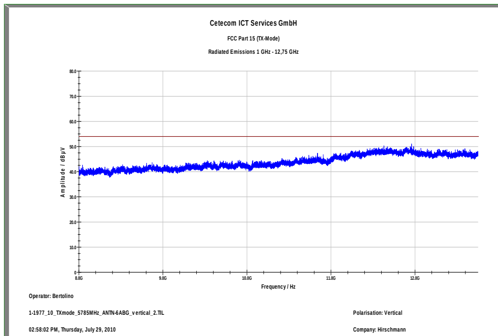
Plot 12: TX mode, mid channel – 5785 MHz, 8 GHz – 12.75 GHz, vertical polarization
