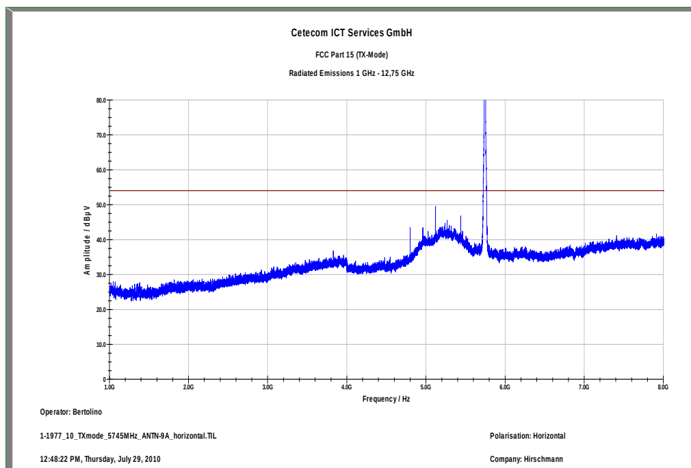
Plot 4: TX mode, low channel – 5745 MHz, 1 GHz – 8 GHz, horizontal polarization
