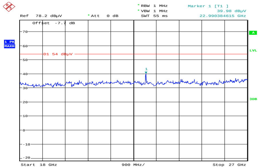
Plot 7: TX mode, low channel – 5745 MHz, 18 GHz – 27 GHz, vertical & horizontal polarization
