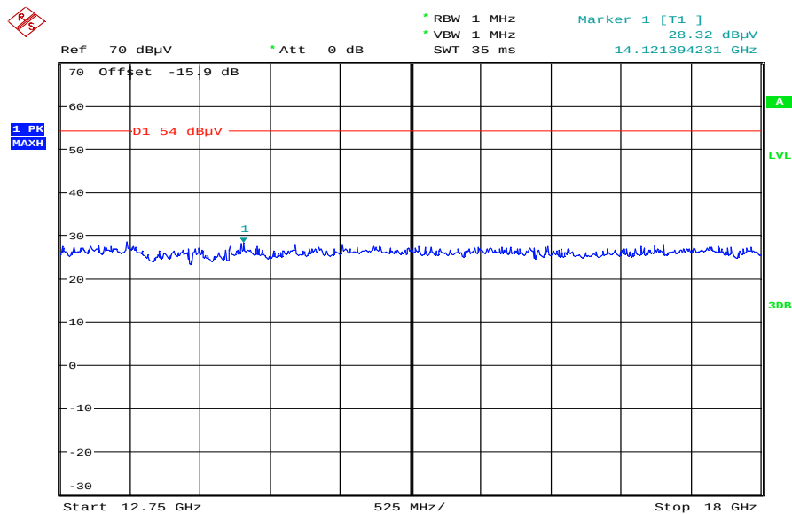
Plot 5: RX mode, 12.75 GHz – 18 GHz, vertical & horizontal polarization
