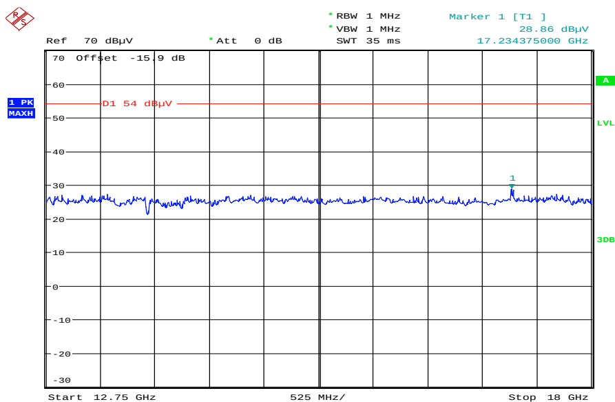
Plot 6: TX mode, low channel – 5745 MHz, 12.75 GHz – 18 GHz, vertical & horizontal polarization
