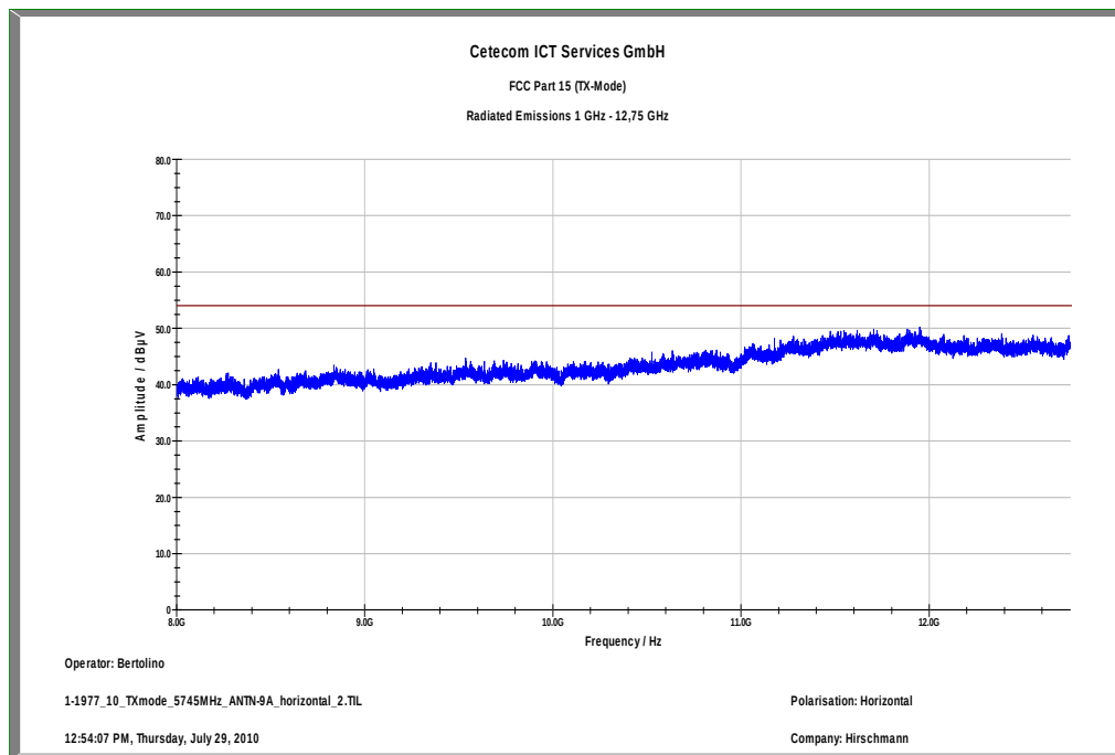
Plot 5: TX mode, low channel – 5745 MHz, 8 GHz – 12.75 GHz, horizontal polarization
