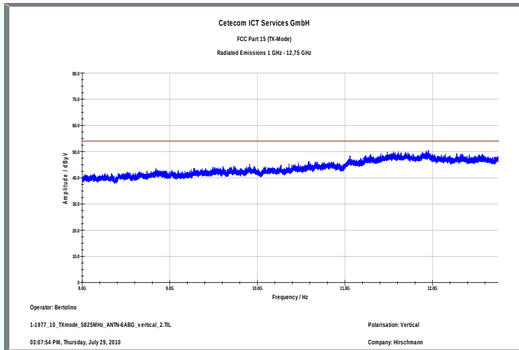
Plot 20: TX mode, high channel – 5825 MHz, 8 GHz – 12.75 GHz, vertical polarization
