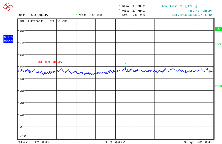
Plot 7: RX mode, 27 GHz – 40 GHz, vertical & horizontal polarization
