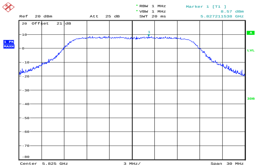
Plot 3: TX mode, high channel – 5825 MHz, power @ 1 MHz
