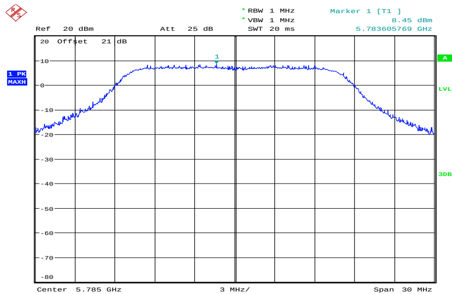
Plot 2: TX mode, mid channel – 5785 MHz, power @ 1 MHz
