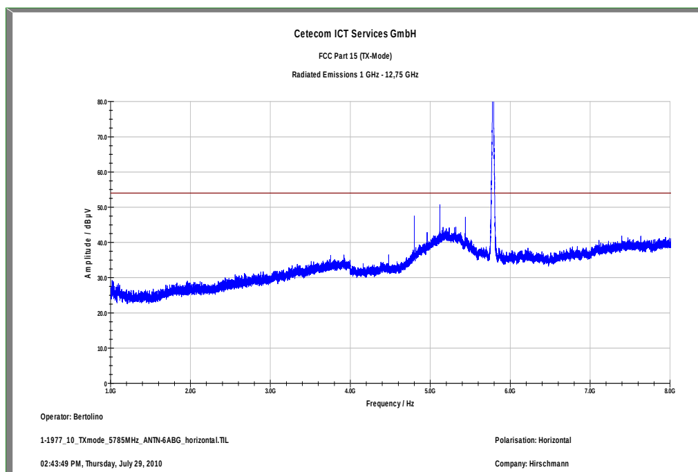
Plot 13: TX mode, mid channel – 5785 MHz, 1 GHz – 8 GHz, horizontal polarization
