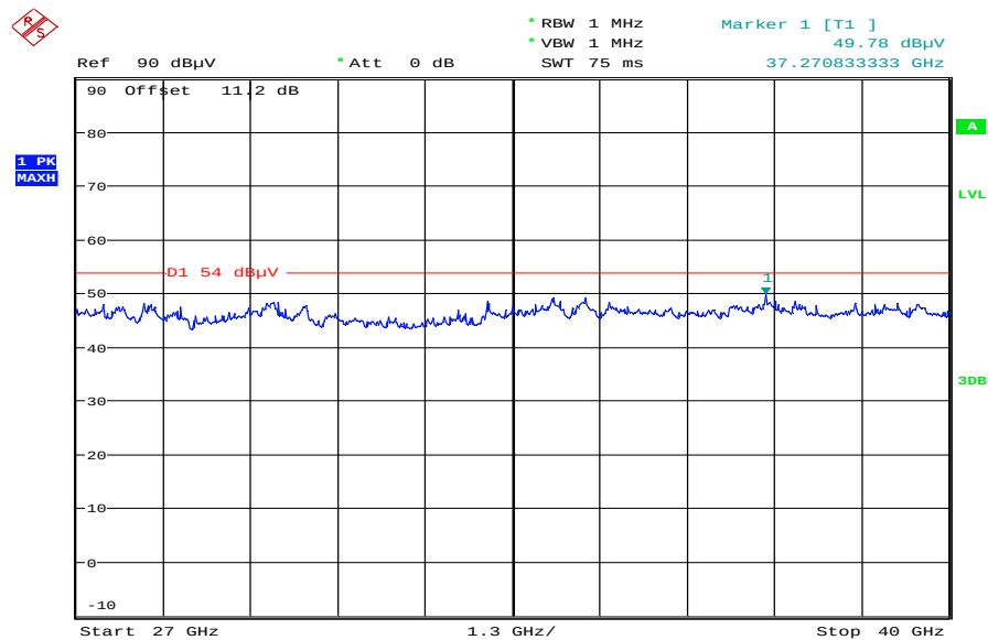
Plot 25: TX mode, high channel – 5825 MHz, 27 GHz – 40 GHz, vertical & horizontal polarization
