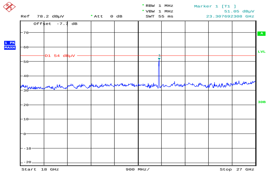
Plot 24: TX mode, high channel – 5825 MHz, 18 GHz – 27 GHz, vertical & horizontal polarization
