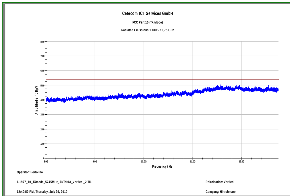
Plot 3: TX mode, low channel – 5745 MHz, 8 GHz – 12.75 GHz, vertical polarization
