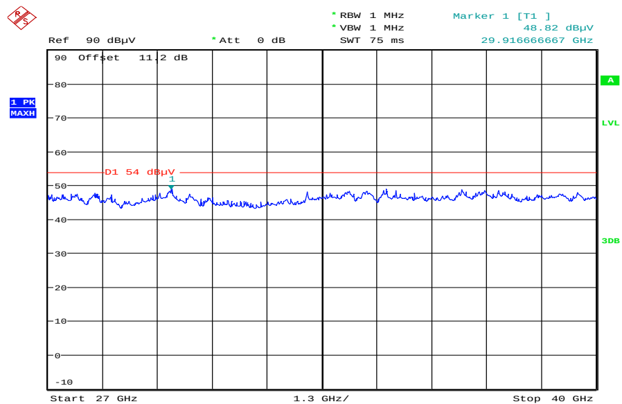
Plot 8: TX mode, low channel – 5745 MHz, 27 GHz – 40 GHz, vertical & horizontal polarization
