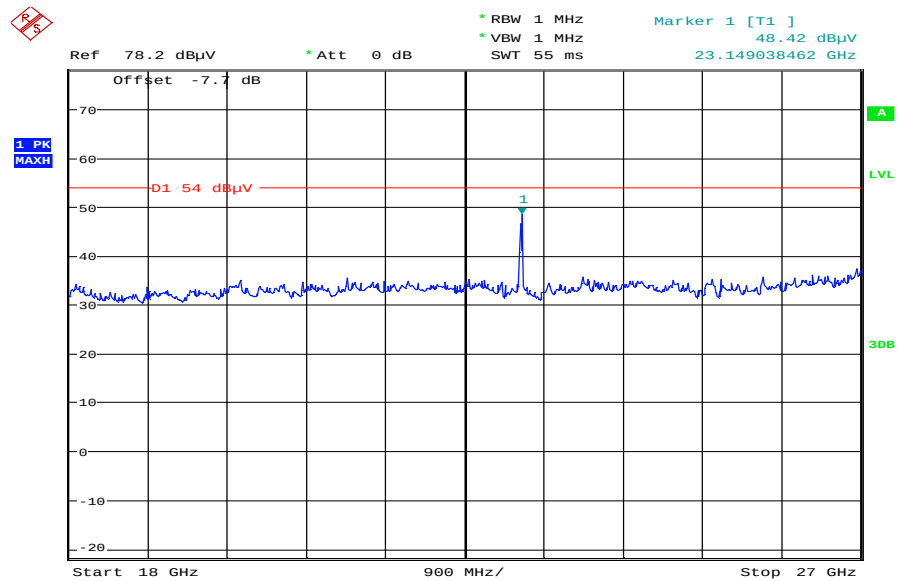
Plot 16: TX mode, mid channel – 5785 MHz, 18 GHz – 27 GHz, vertical & horizontal polarization
