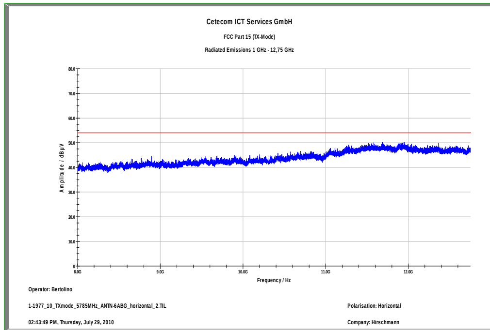
Plot 14: TX mode, mid channel – 5785 MHz, 8 GHz – 12.75 GHz, horizontal polarization
