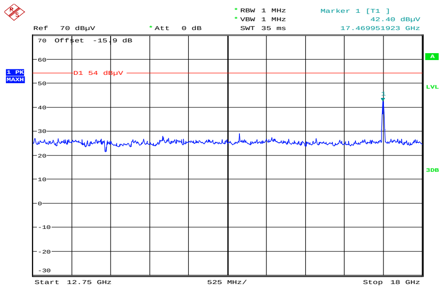
Plot 23: TX mode, high channel – 5825 MHz, 12.75 GHz – 18 GHz, vertical & horizontal polarization
