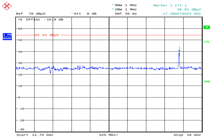
Plot 15: TX mode, mid channel – 5785 MHz, 12.75 GHz – 18 GHz, vertical & horizontal polarization
