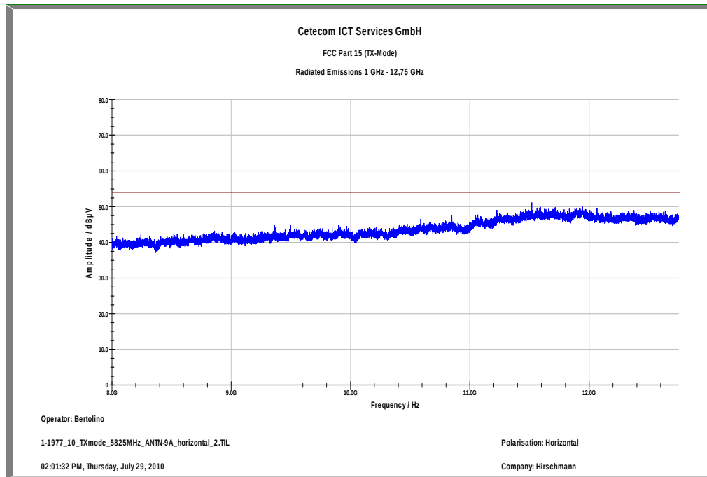
Plot 22: TX mode, high channel – 5825 MHz, 8 GHz – 12.75 GHz, horizontal polarization
