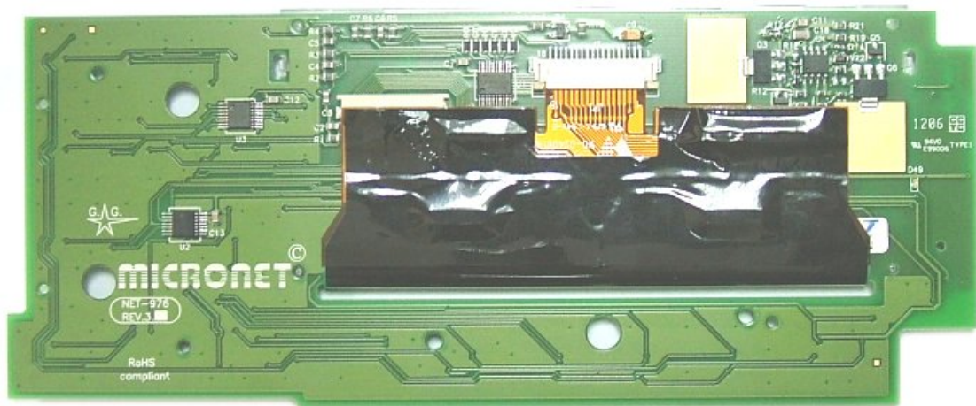
Figure 5 Keyboard PCB Side 2
