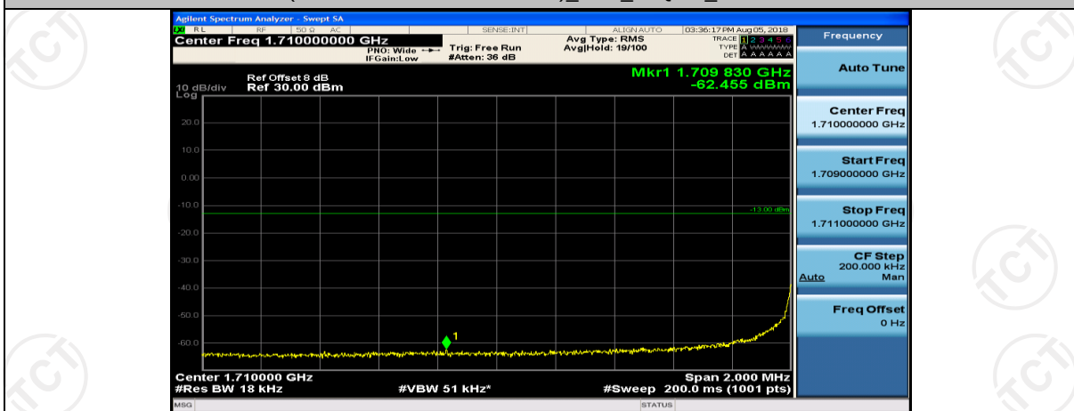
(Channel Bandwidth:20 MHz)_LCH_16QAM_50RB#0
