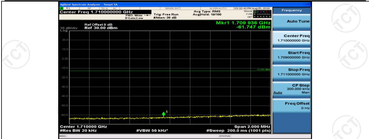
(Channel Bandwidth:15 MHz)_LCH_QPSK_1RB#74
