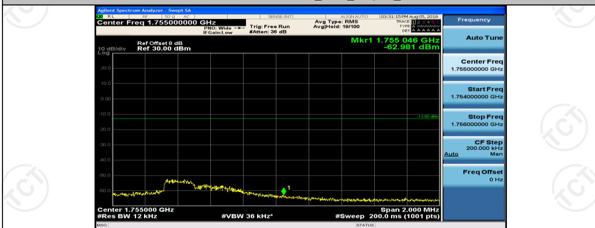
Channel Bandwidth: 10 MHz_HCH_16QAM_1RB#24
