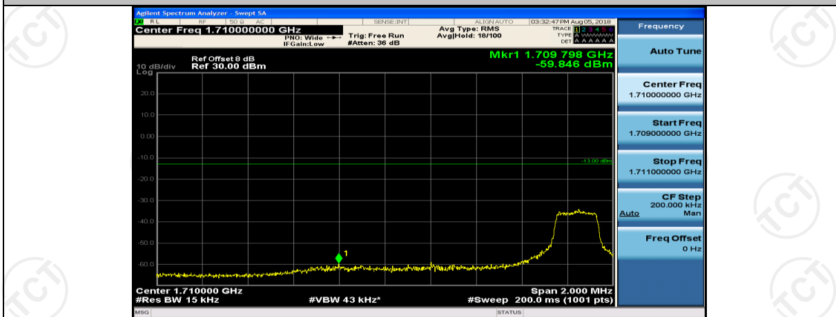
(Channel Bandwidth:15 MHz)_LCH_QPSK_37RB#0
