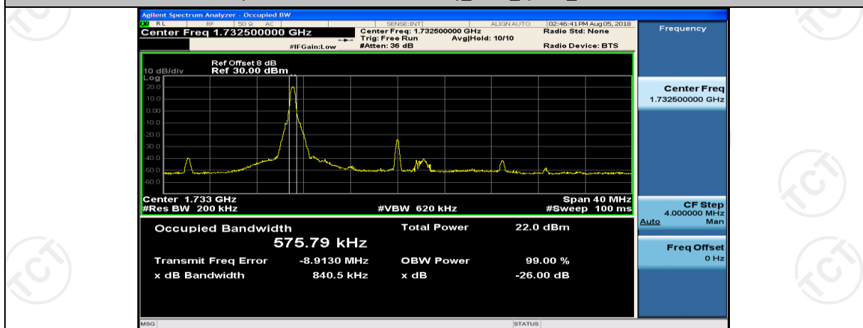
(Channel Bandwidth:20 MHz)_MCH_QPSK_1RB#50
