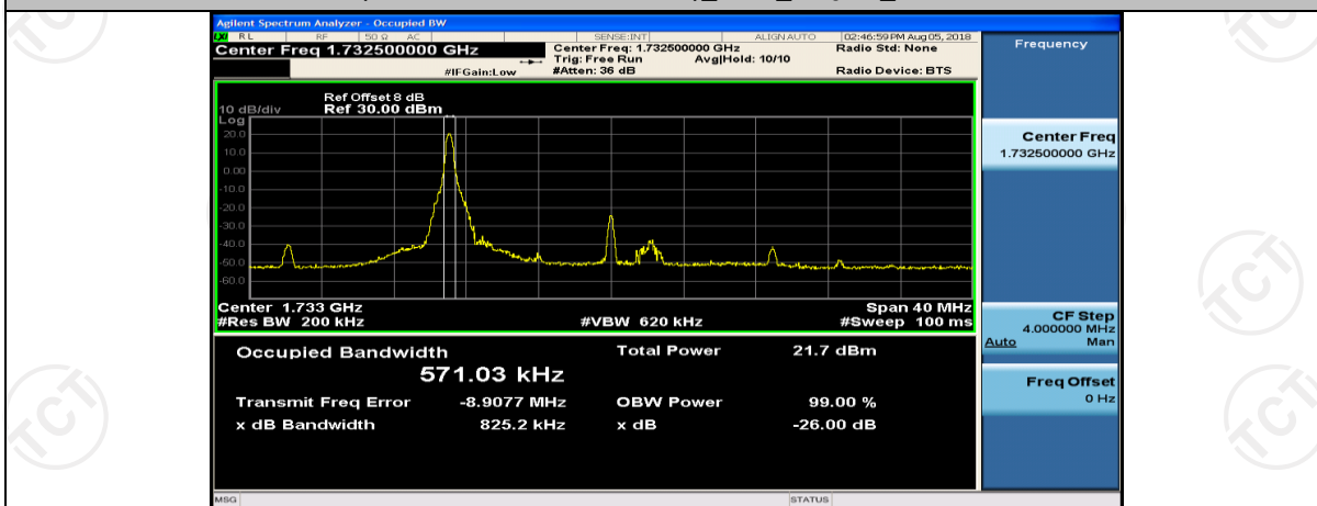
(Channel Bandwidth:20 MHz)_MCH_16QAM_1RB#50
