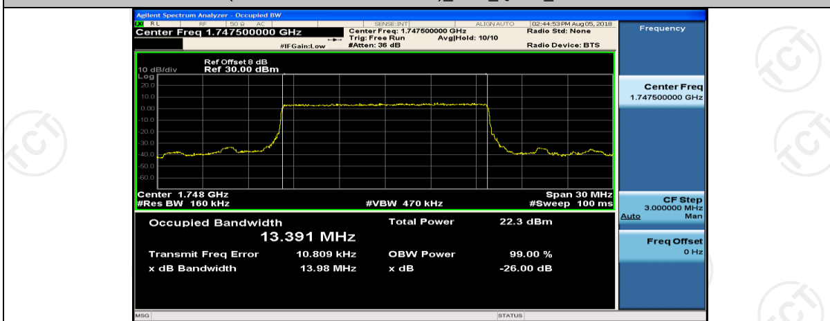
(Channel Bandwidth:15 MHz)_HCH_QPSK_75RB#0
