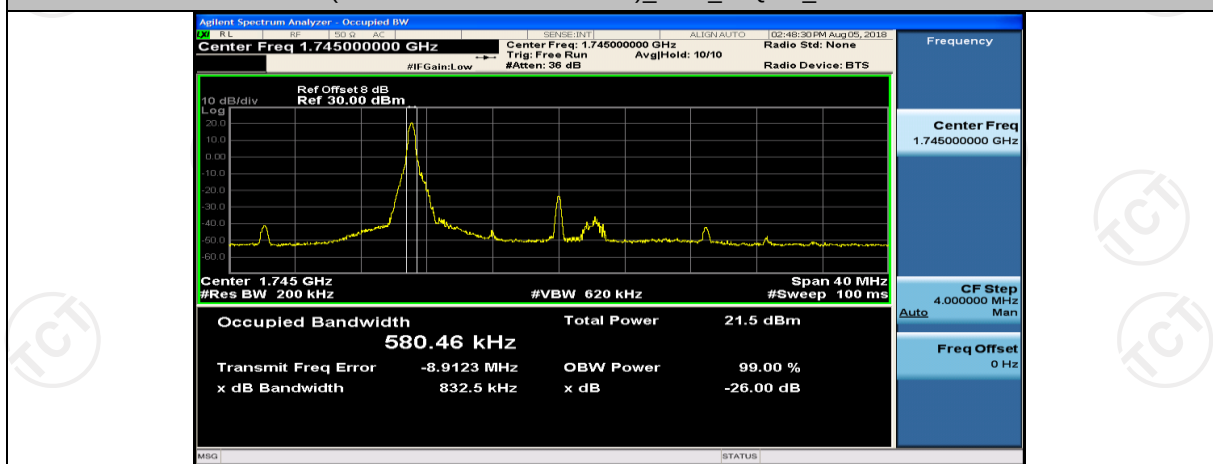
(Channel Bandwidth:20 MHz)_HCH_16QAM_1RB#50
