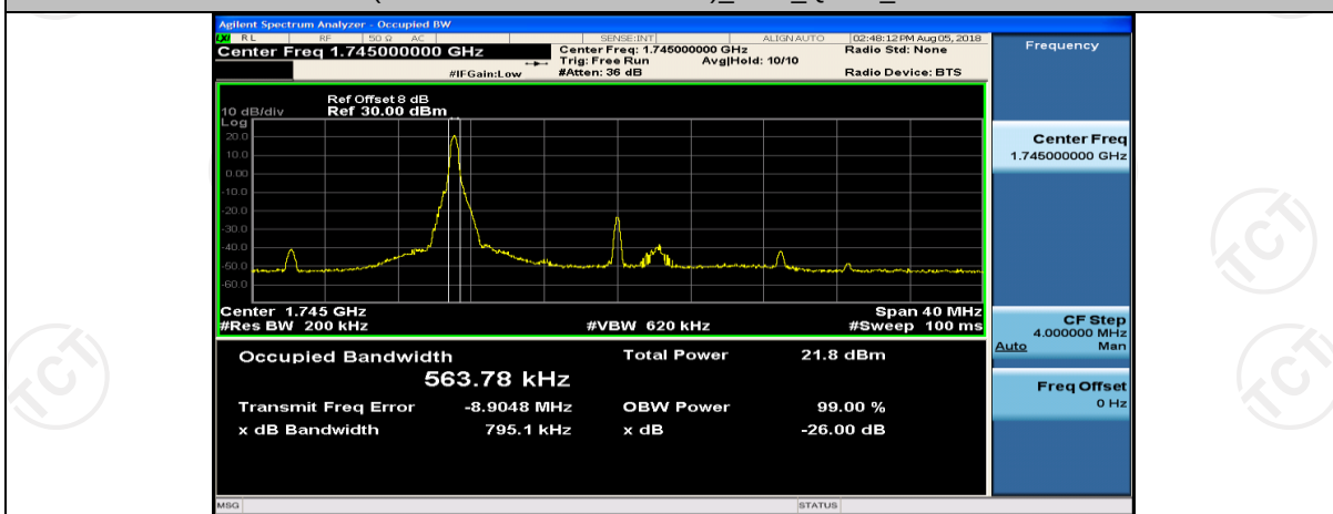
(Channel Bandwidth:20 MHz)_HCH_QPSK_1RB#50
