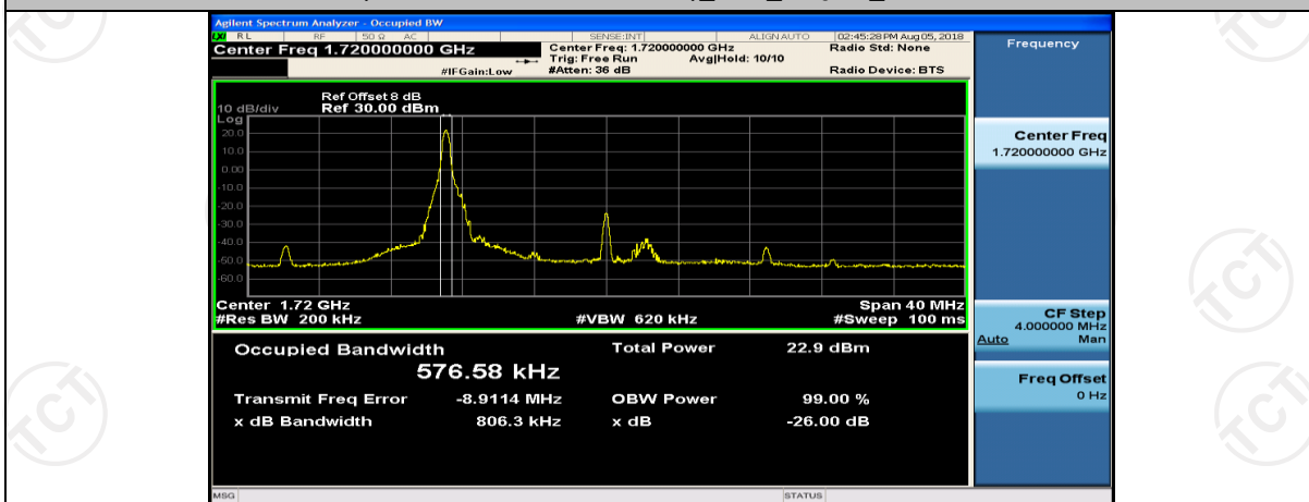
(Channel Bandwidth:20 MHz)_LCH_16QAM_1RB#50
