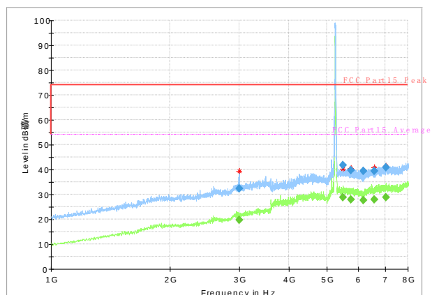
Radiated Spurious Emission (802.11n-HT40, ch46, 1GHz-8GHz)
