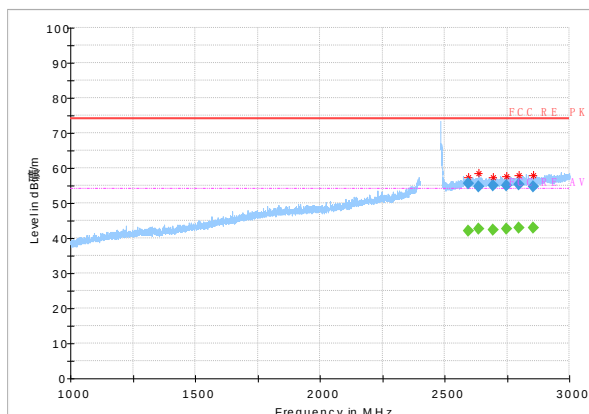
Radiated Spurious Emission (802.11g, Ch11, 1GHz~3GHz)
