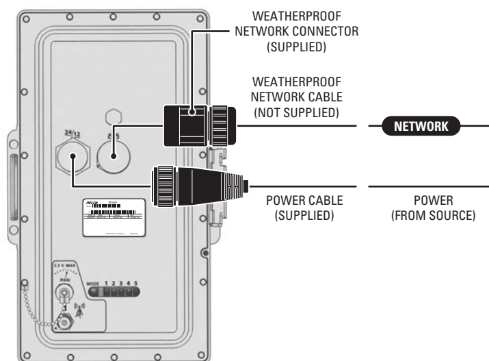
Figure 5. Sample Installation for Separate Power and Network Cables
