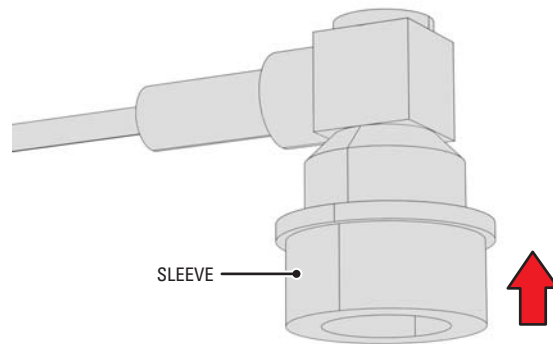
Figure 15. Disconnecting an Antenna Cable Connector
