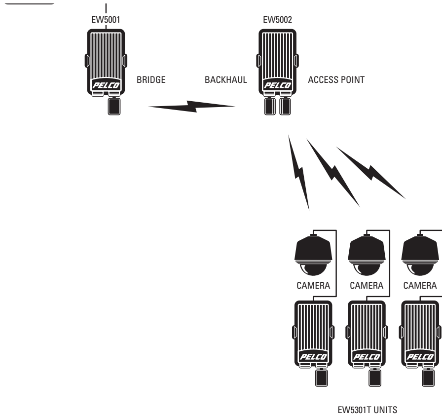
Figure 3. Sample EW5001 Wireless Bridge Application Scenario
