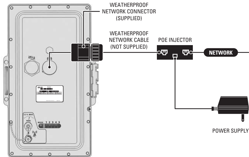
Figure 6. PoE Injector Configuration
