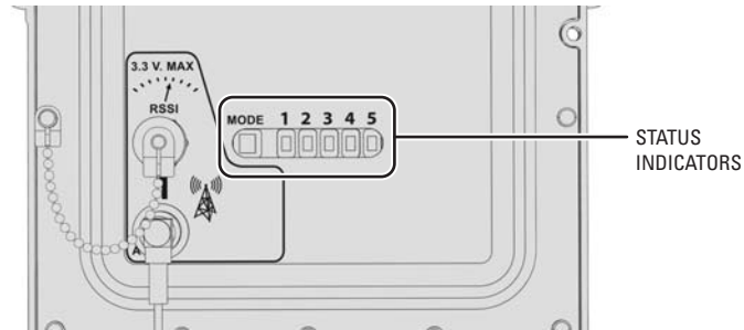
Figure 18. EW5001 Status Indicators
