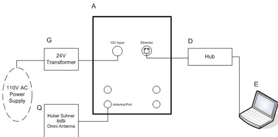
Figure 2. Block Diagram of Test Configuration (Conducted Emissions, 5301, 12VDC)
