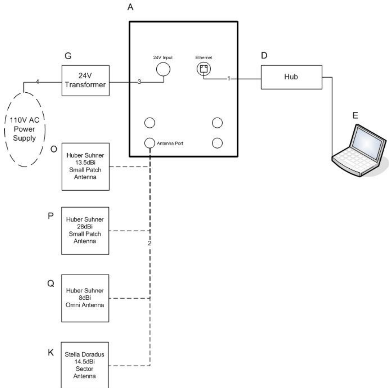
Figure 7. Block Diagram of Test Configuration (XR5 Antenna Configuration)
