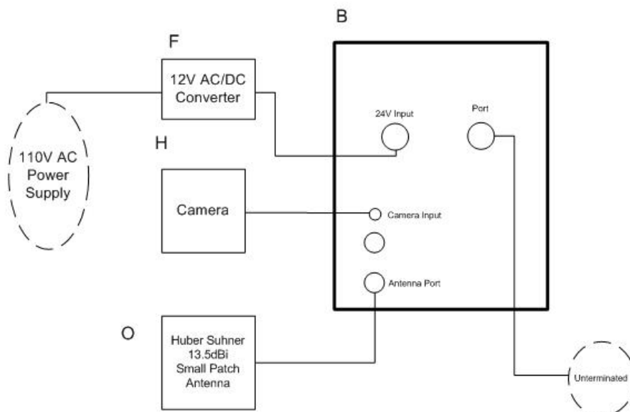
Figure 3. Block Diagram of Test Configuration (Conducted Emissions, 5002, 24VAC)
