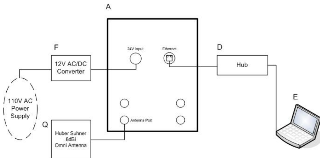
Figure 4. Block Diagram of Test Configuration (Conducted Emissions, 5301, 24VAC)
