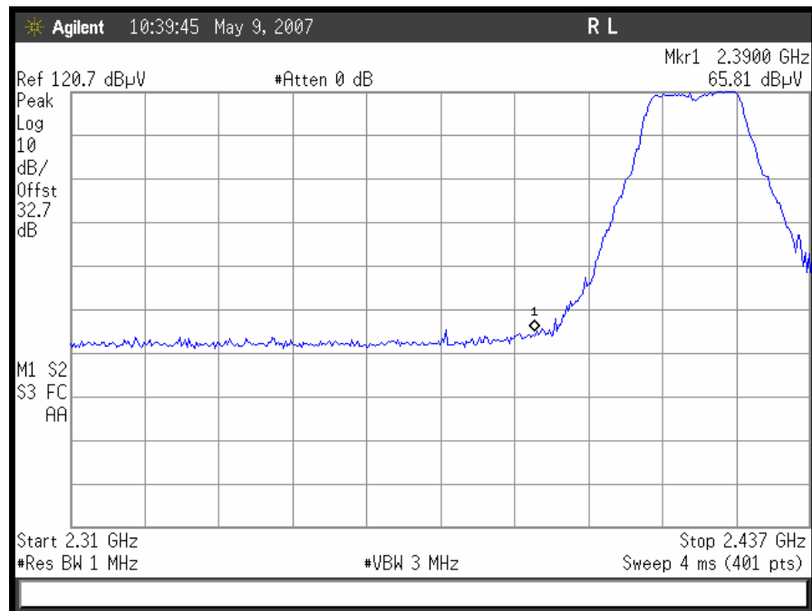
802.11/g radiated restricted band 2310- 2437 MHz Peak (Channel 2)
