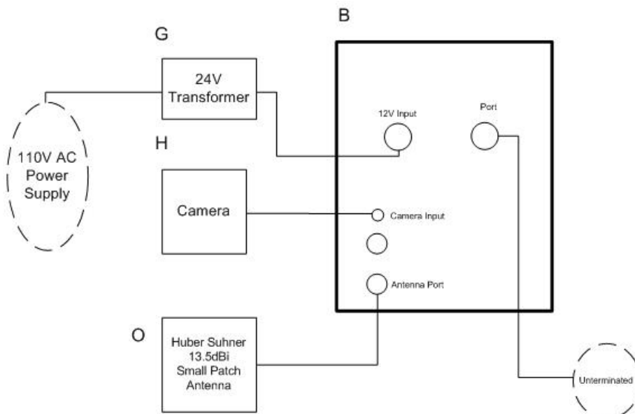
Figure 1. Block Diagram of Test Configuration (Conducted Emissions, 5002, 12VDC)
