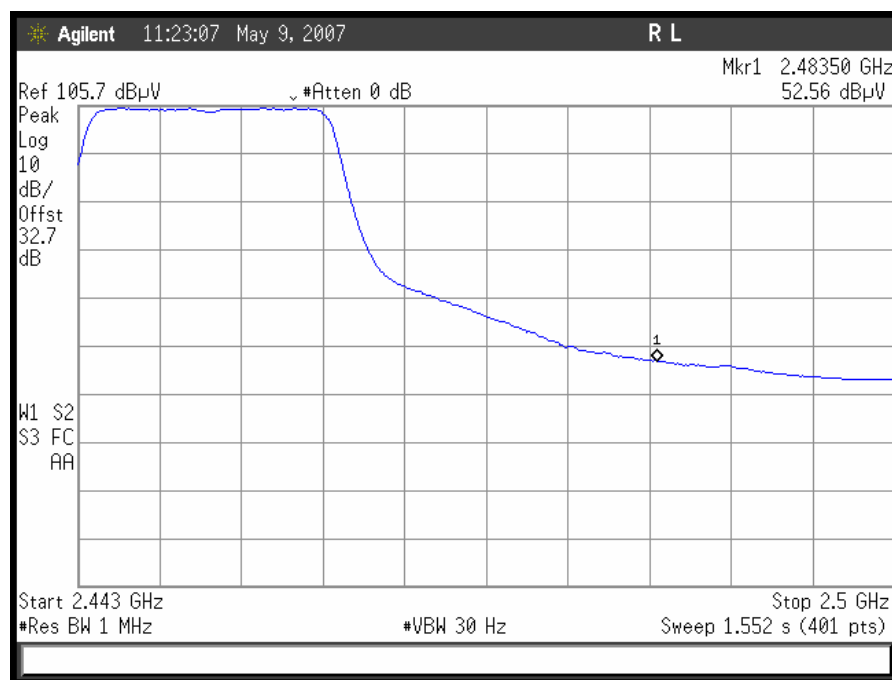
802.11/g radiated restricted band 2443 – 2500MHz Avg (Channel 9)
