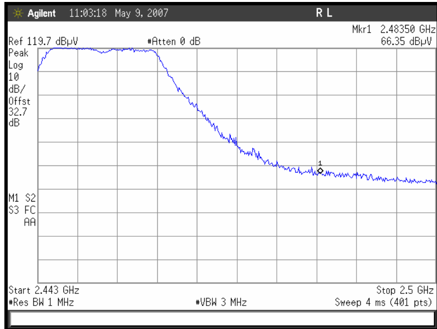
802.11/g radiated restricted band 2443 – 2500MHz Peak (Channel 9)
