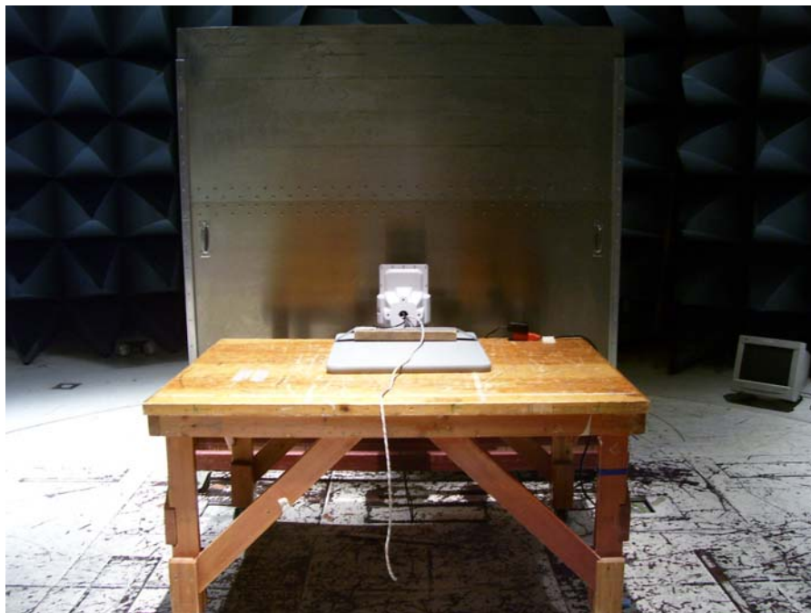
Photograph 14. Conducted Emissions Test Setup, EW 5301 CEV w 12V DC PSU (Front)
