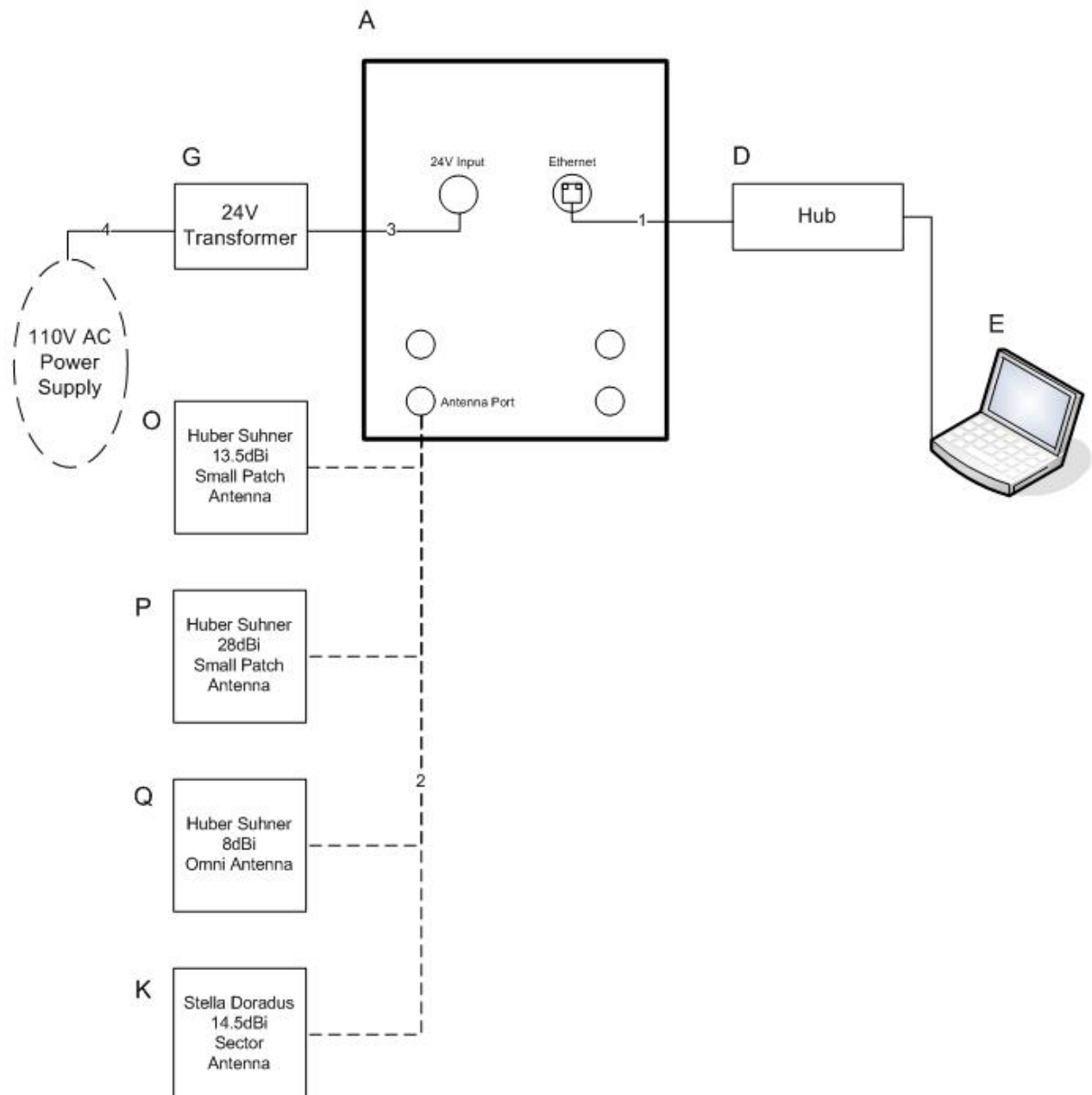
Figure 6. Block Diagram of Test Configuration (SR5 Antenna Configuration)
