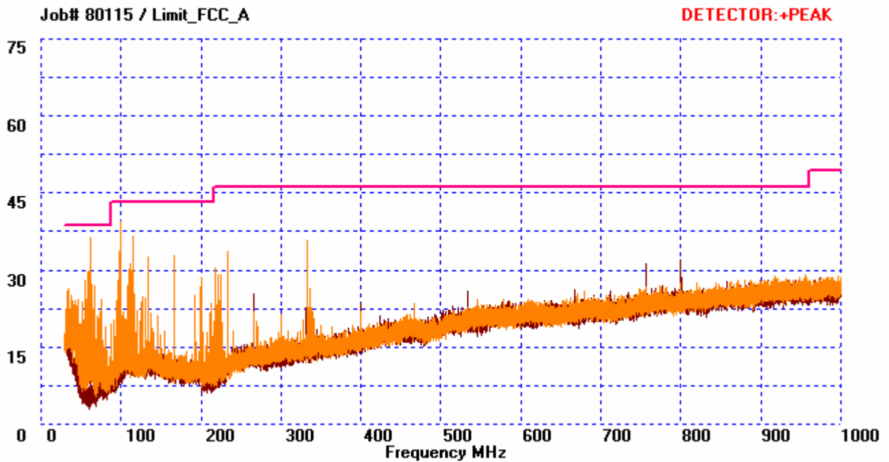
Radiated Emissions Limits Plot, 30 MHz – 1 GHz, Class A
