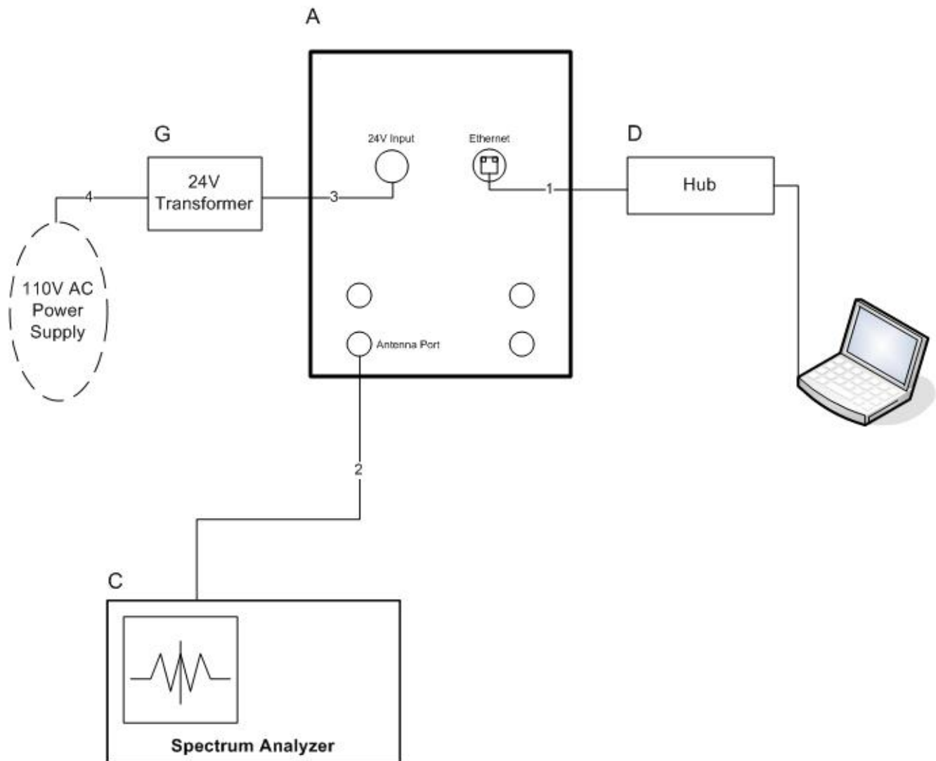
Figure 9. Block Diagram of Test Configuration (Conducted Measurement)
