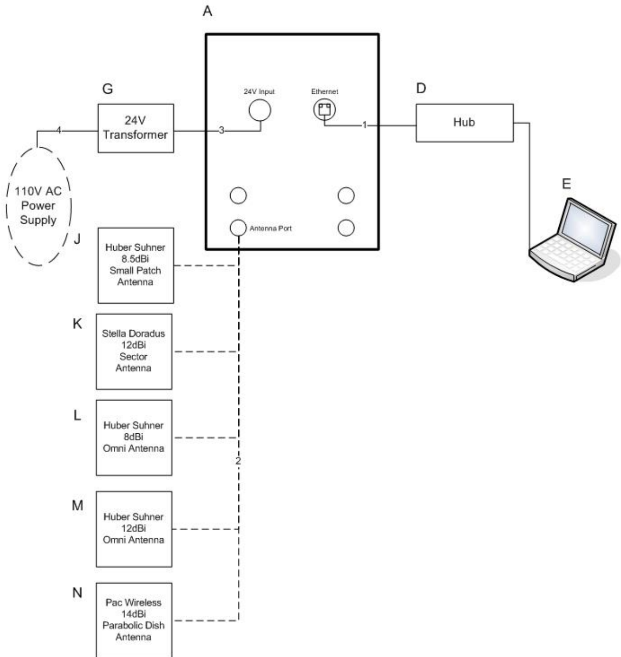
Figure 8. Block Diagram of Test Configuration (XR2 Antenna Configuration)
