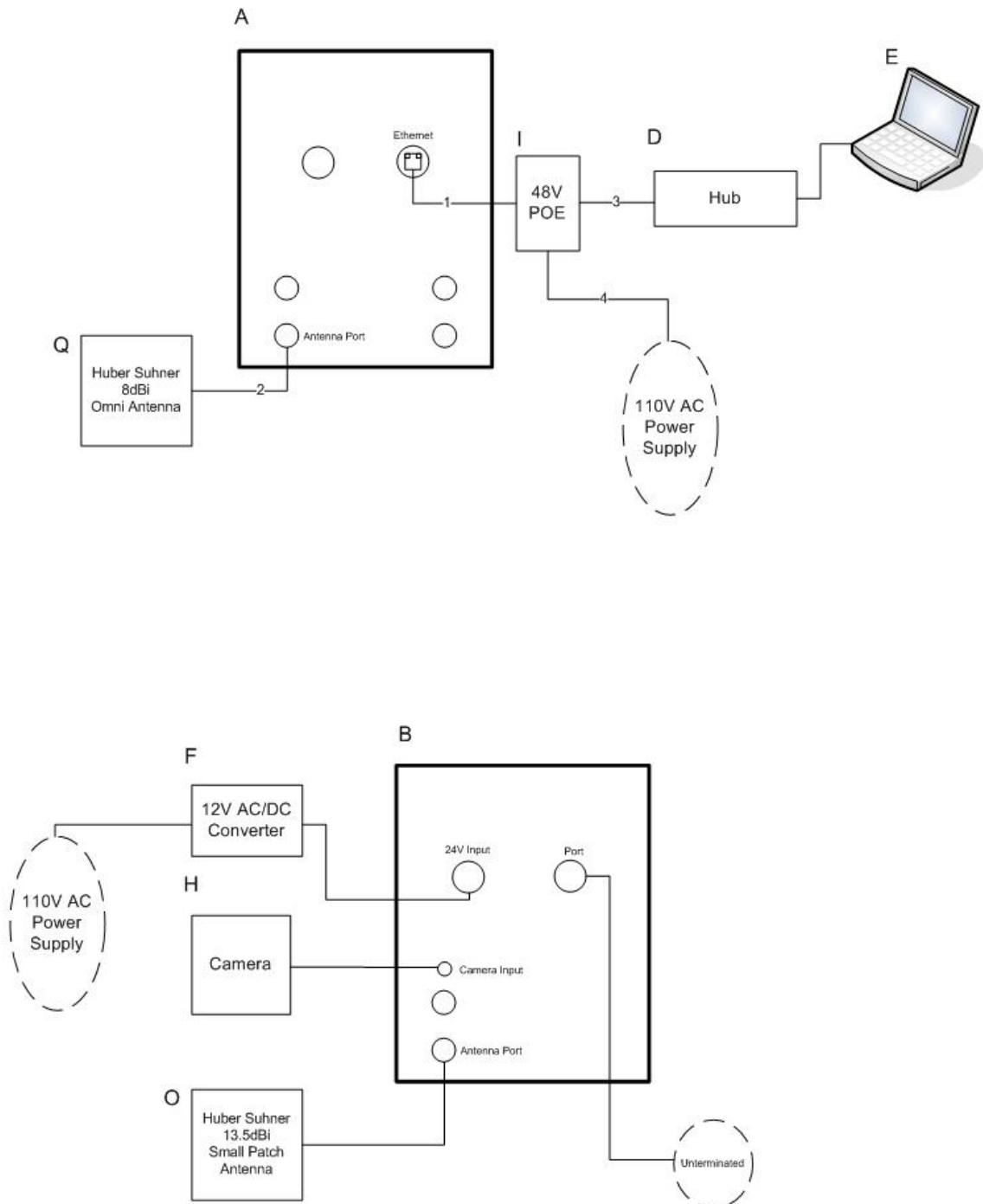
Figure 5. Block Diagram of Test Configuration (Conducted Emissions, 5002, 48V POE)
