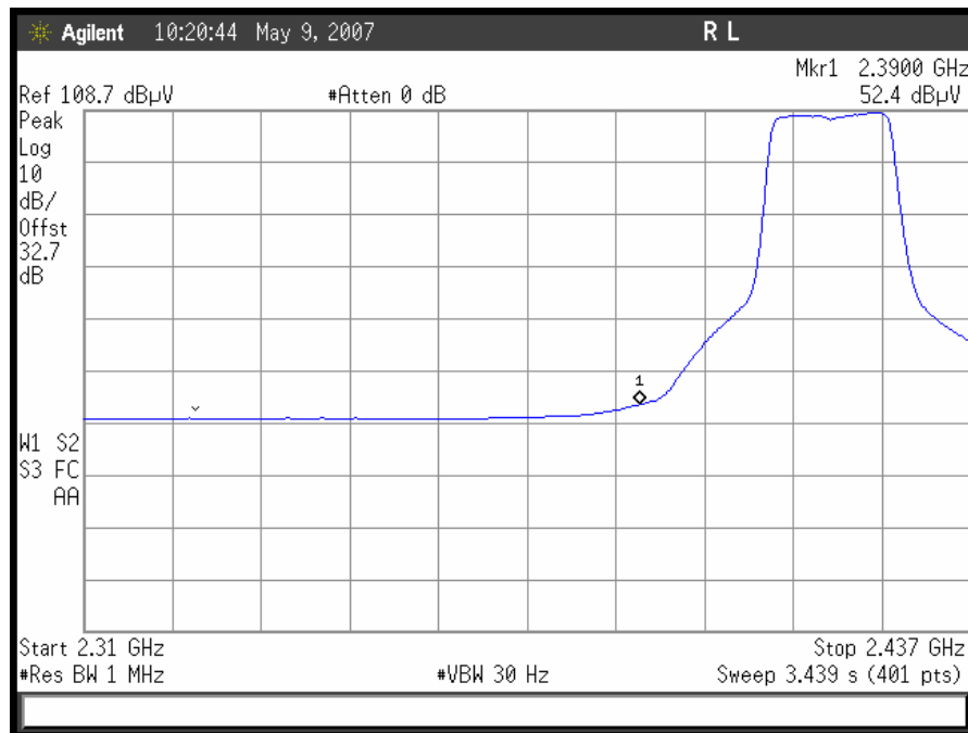
802.11/g radiated restricted band 2310- 2437 MHz Avg (Channel 2)
