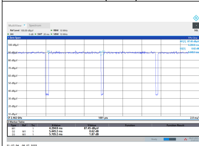
802.11ax (20 MHz)
