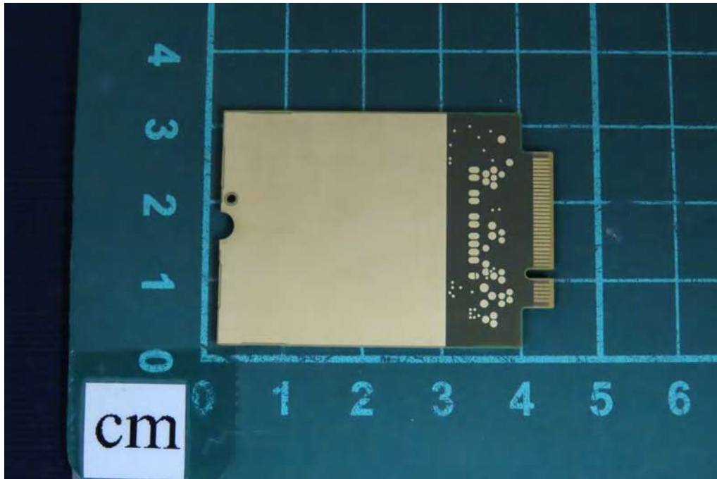
(8) EUT Photo (WWAN module: Telit / LE910C4-NF)
