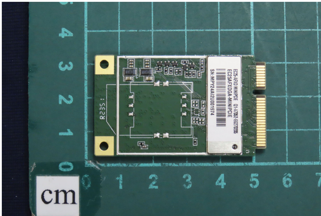
(7) EUT Photo
