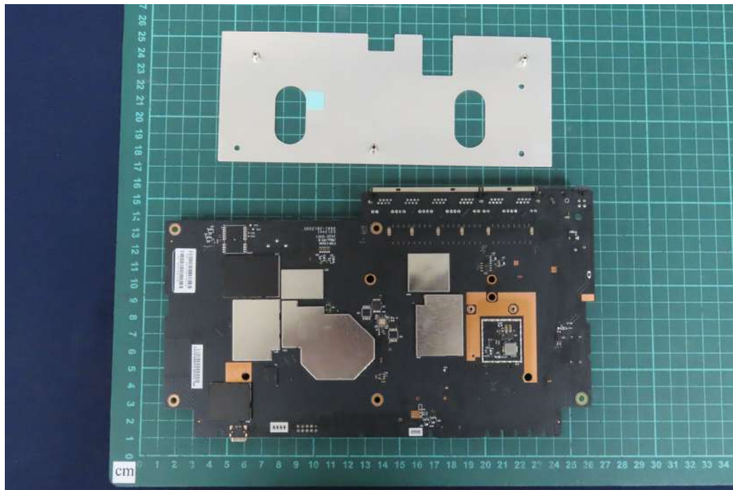
(45) EUT Photo
