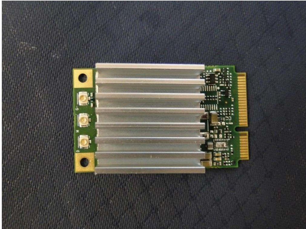
(21) EUT Photo _ Module: LE910C4-NF
