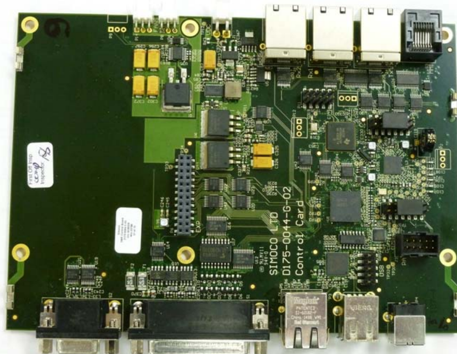
SDB680 Control Board Top
