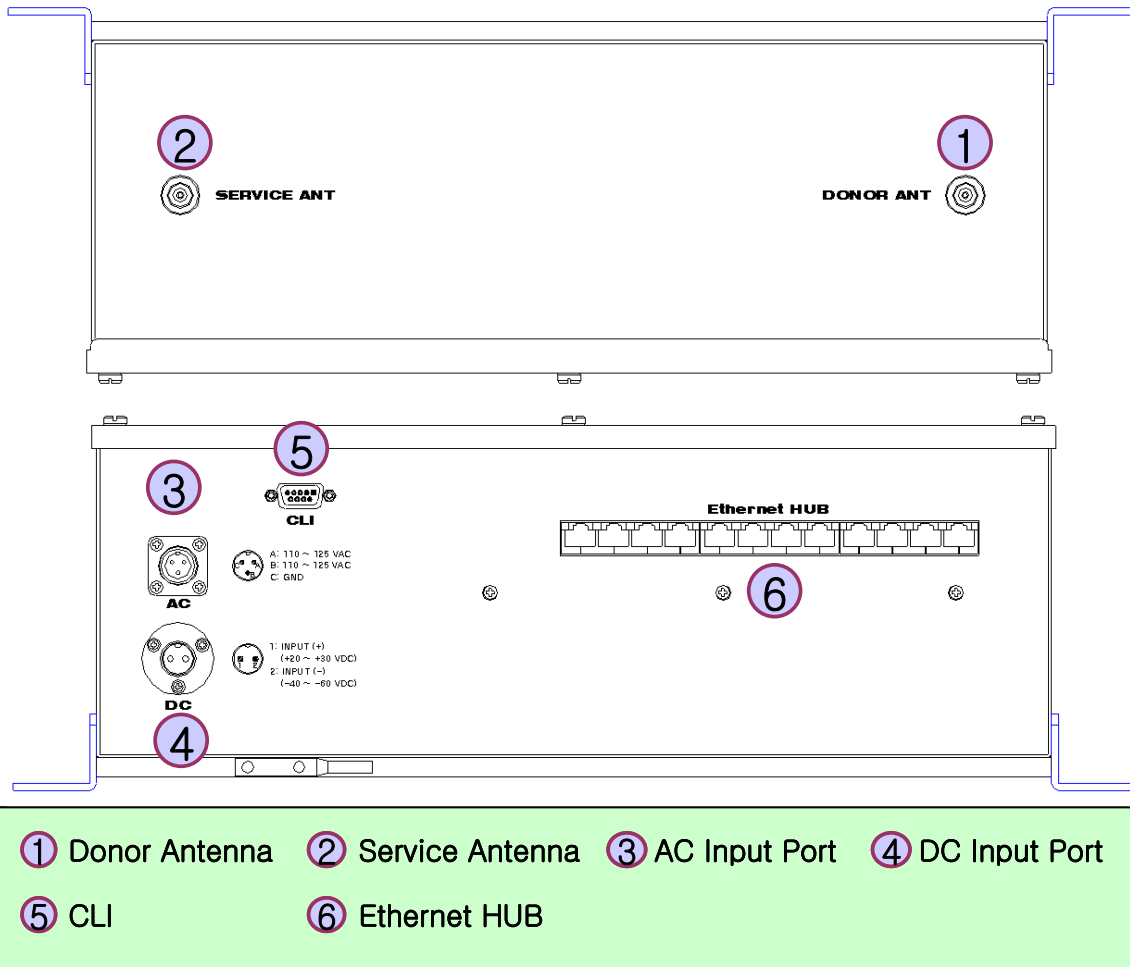
<Pic.3> Repeater's Top and Bottom panels
