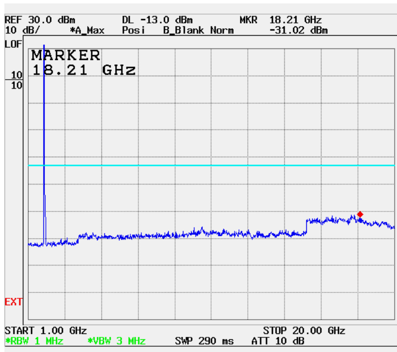
Conducted Spurious Emissions Uplink Low CH (1 GHz – 20 GHz)
