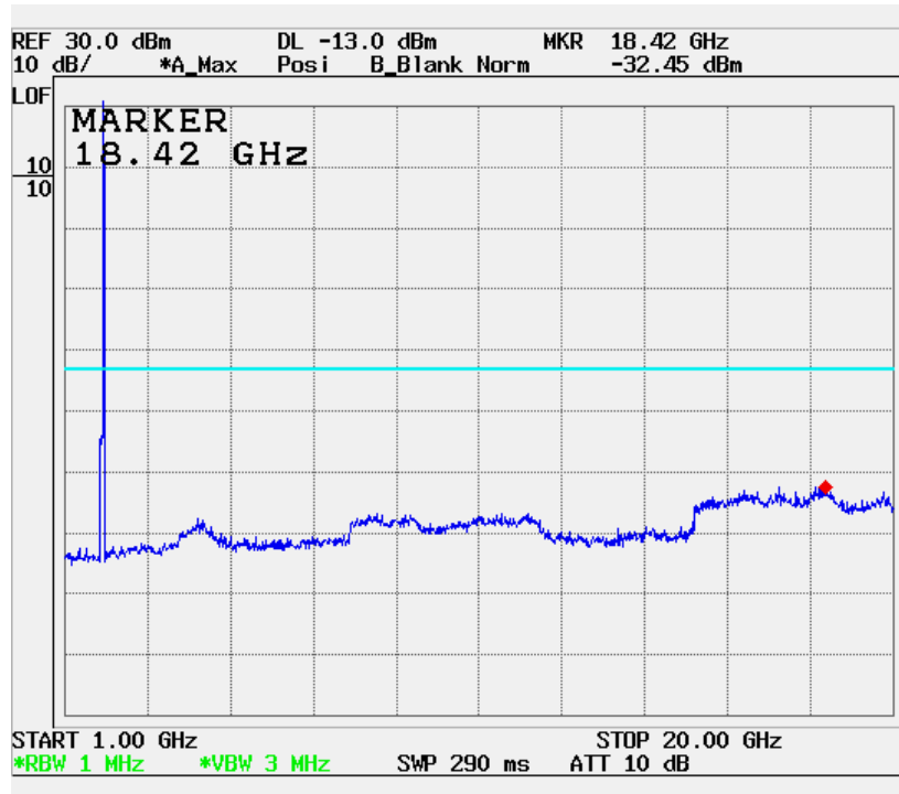
Conducted Spurious Emissions Uplink Mid CH (1 GHz – 20 GHz)
