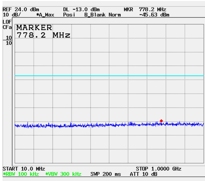
Conducted Spurious Emissions Uplink Mid CH (10 MHz – 1 GHz)
