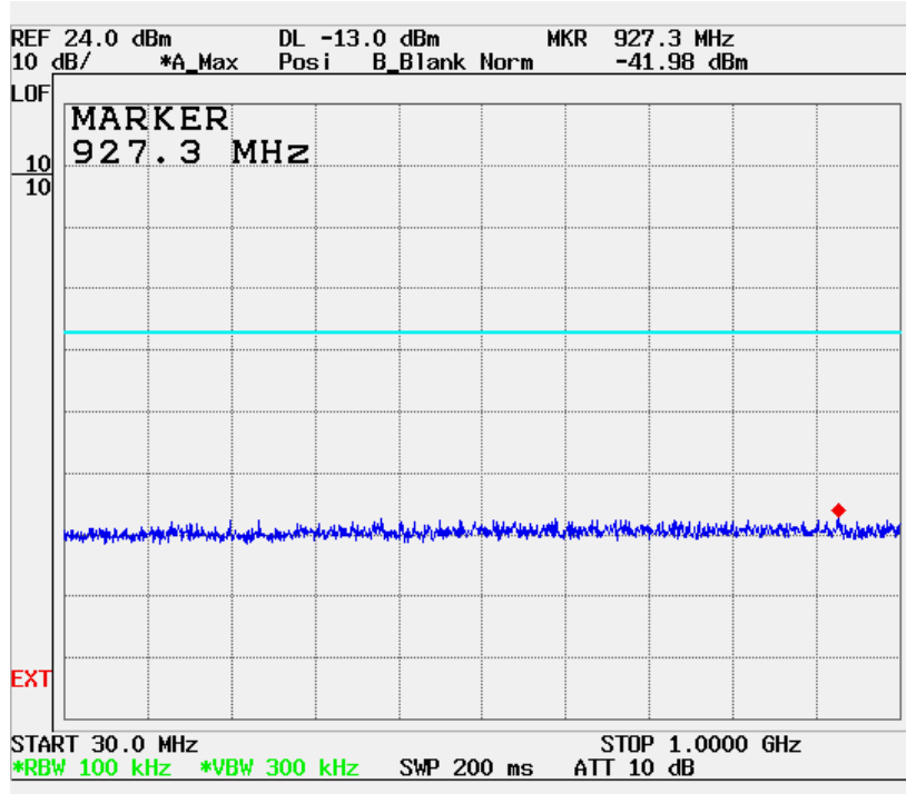
Conducted Spurious Emissions Uplink Low CH (30 MHz – 1 GHz)
