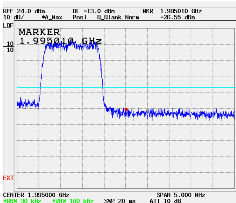
(CDMA Downlink High CH)
