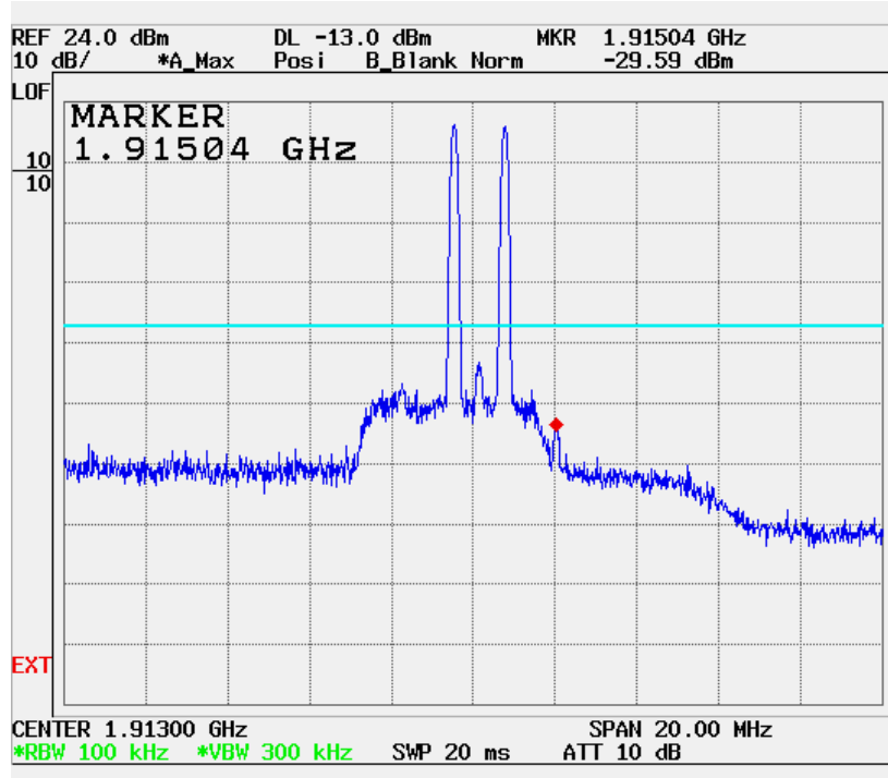
Two Tone Uplink High End Intermodulation
