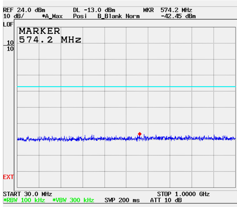
Conducted Spurious Emissions Uplink High CH (30 MHz – 1 GHz)
