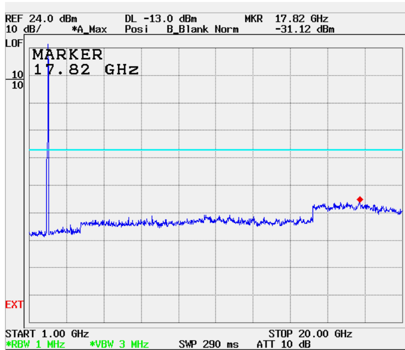
Conducted Spurious Emissions Downlink High CH (1 GHz – 20 GHz)
