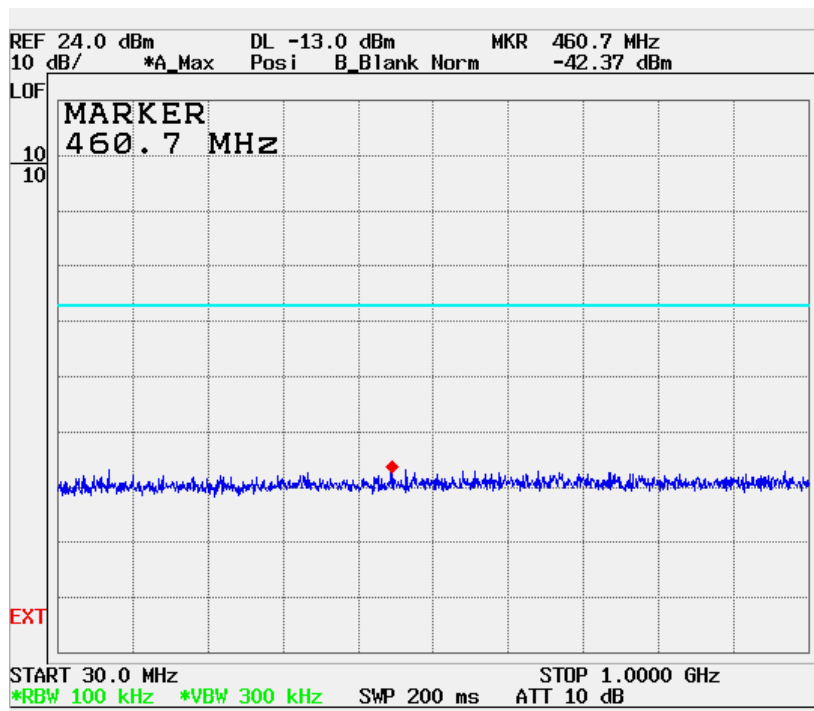
Conducted Spurious Emissions Downlink Low CH (30 MHz – 1 GHz)
