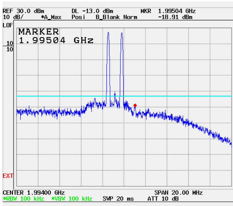
Two Tone Downlink High End Intermodulation
