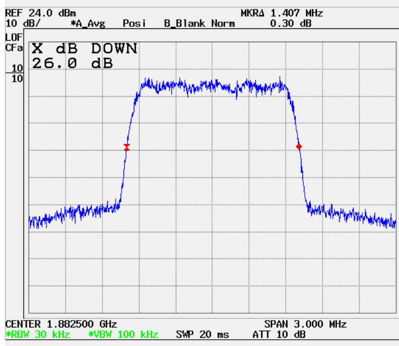
CDMA Uplink MidCH Output
