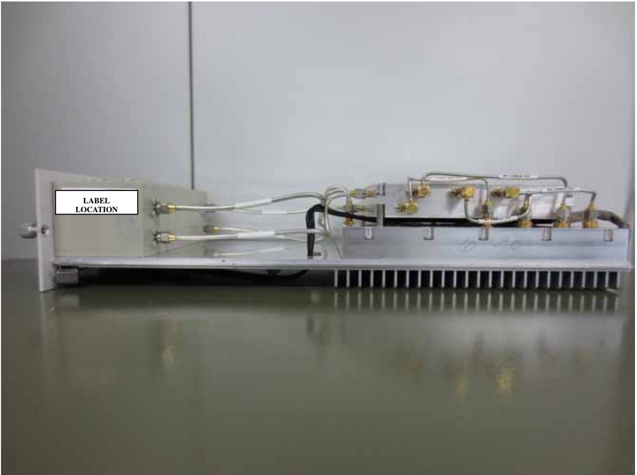
Figure 1.2 LABEL LOCATION
