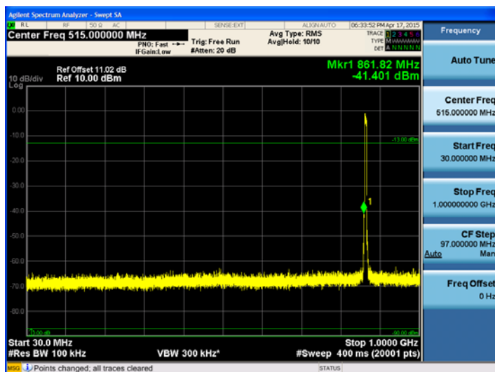
800 MHz band (30 MHz – 1 GHz) LTE 5MHz
