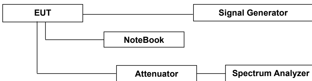
Block Diagram 1. RF Power Output Test Setup
