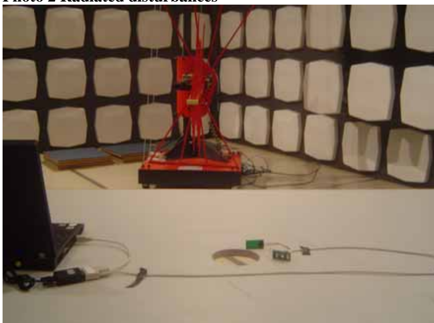
Photo 2 Radiated disturbances
