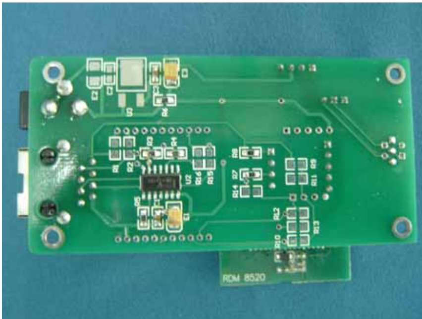
Photo 8 Mainboard & RF pcb of the EUT
