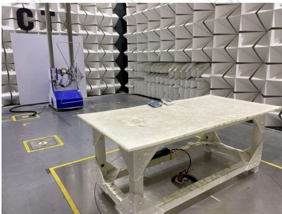
Radiated spurious emission Test Setup-2(Below 1G)
