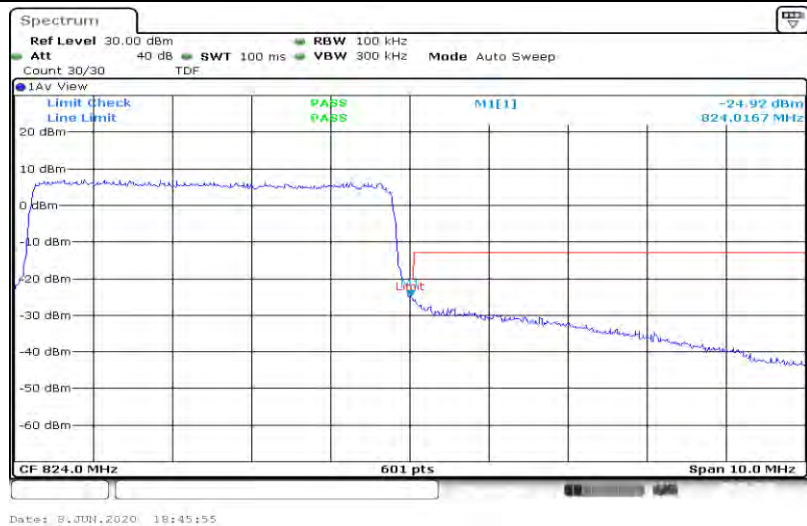
Band26-5MHz-16QAM-26815-25RB#0
