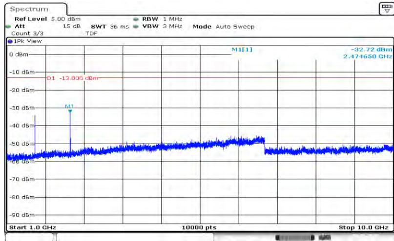
Band26-1.4MHz-16QAM-26797-6RB#0-Range2:1000~10000MHz
