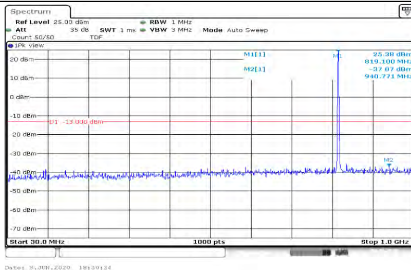
Band26-1.4MHz-QPSK-26740-6RB#0-Range1:30~1000MHz
