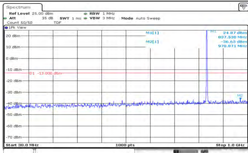
Band26-1.4MHz-16QAM-26915-6RB#0-Range1:30~1000MHz
