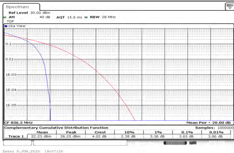
Band26-1.4MHz-QPSK-27033-6RB#0
