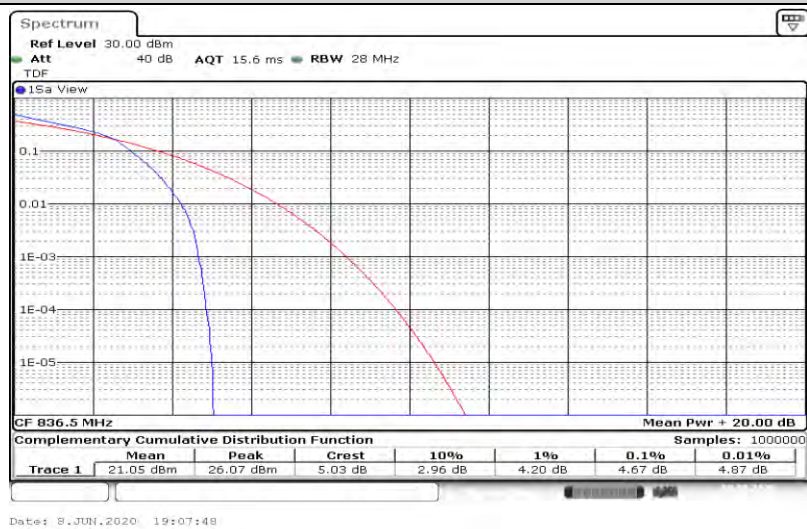
Band26-1.4MHz-16QAM-27033-6RB#0
