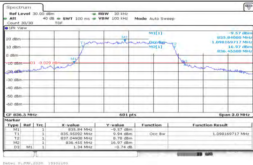
Band26-1.4MHz-QPSK-27033-6RB#0-1.098
