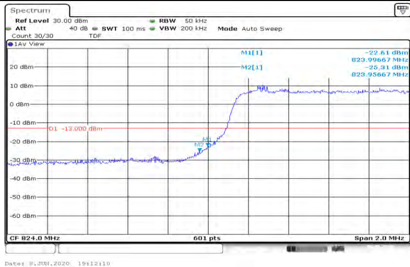
Band26-3MHz-QPSK-27025-15RB#0
