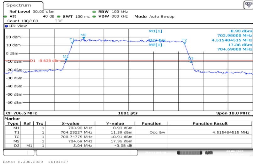
Band17-5MHz-QPSK-23790-25RB#0-4.515
