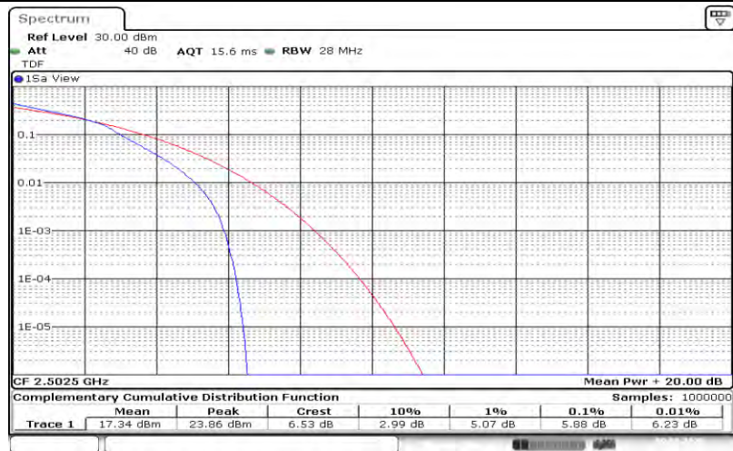
Band7-5MHz-16QAM-20775-25RB#0
