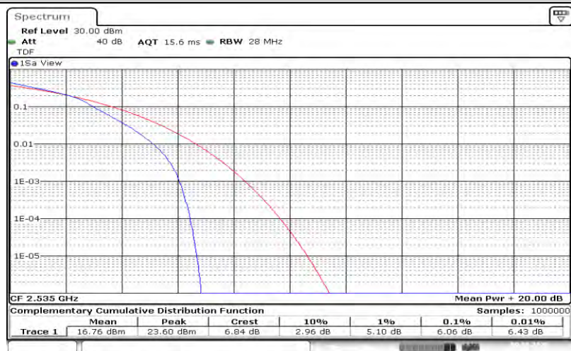
Band7-5MHz-16QAM-21100-25RB#0
