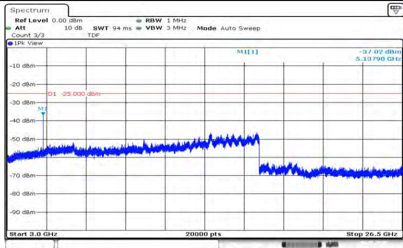
Band7-5MHz-16QAM-21425-25RB#0-Range3:3000~26500MHz
