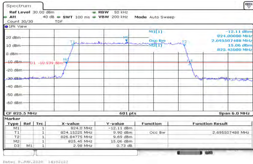
Band5-3MHz-16QAM-20525-15RB#0-2.696
