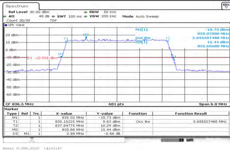
Band5-3MHz-16QAM-20635-15RB#0-2.696
