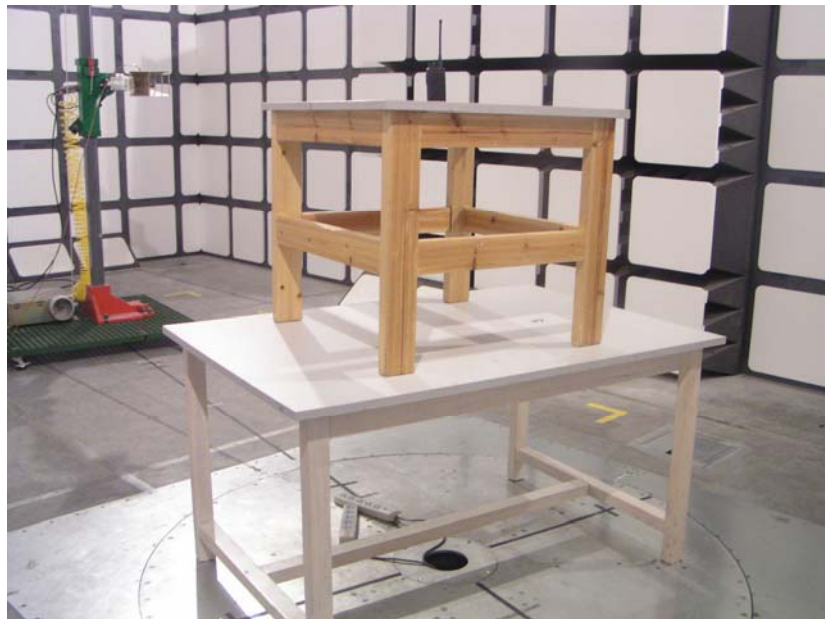
Radiated Emissions - Rear View (Above 1000 MHz)
