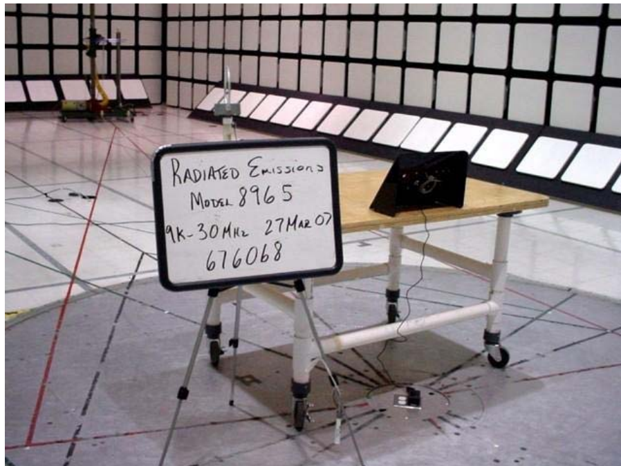
Radiated Emissions 10kHz-30MHz
