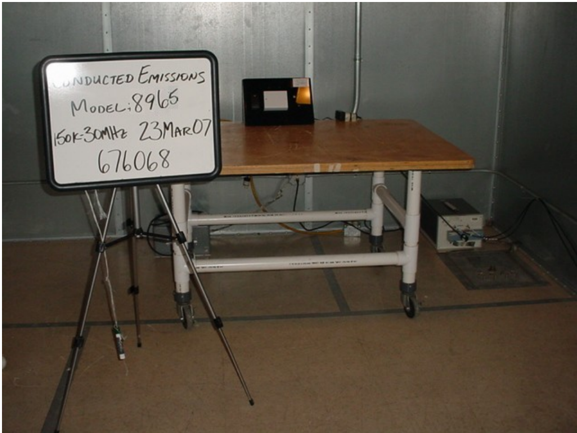
Conducted Emissions 150kHz-30MHz
