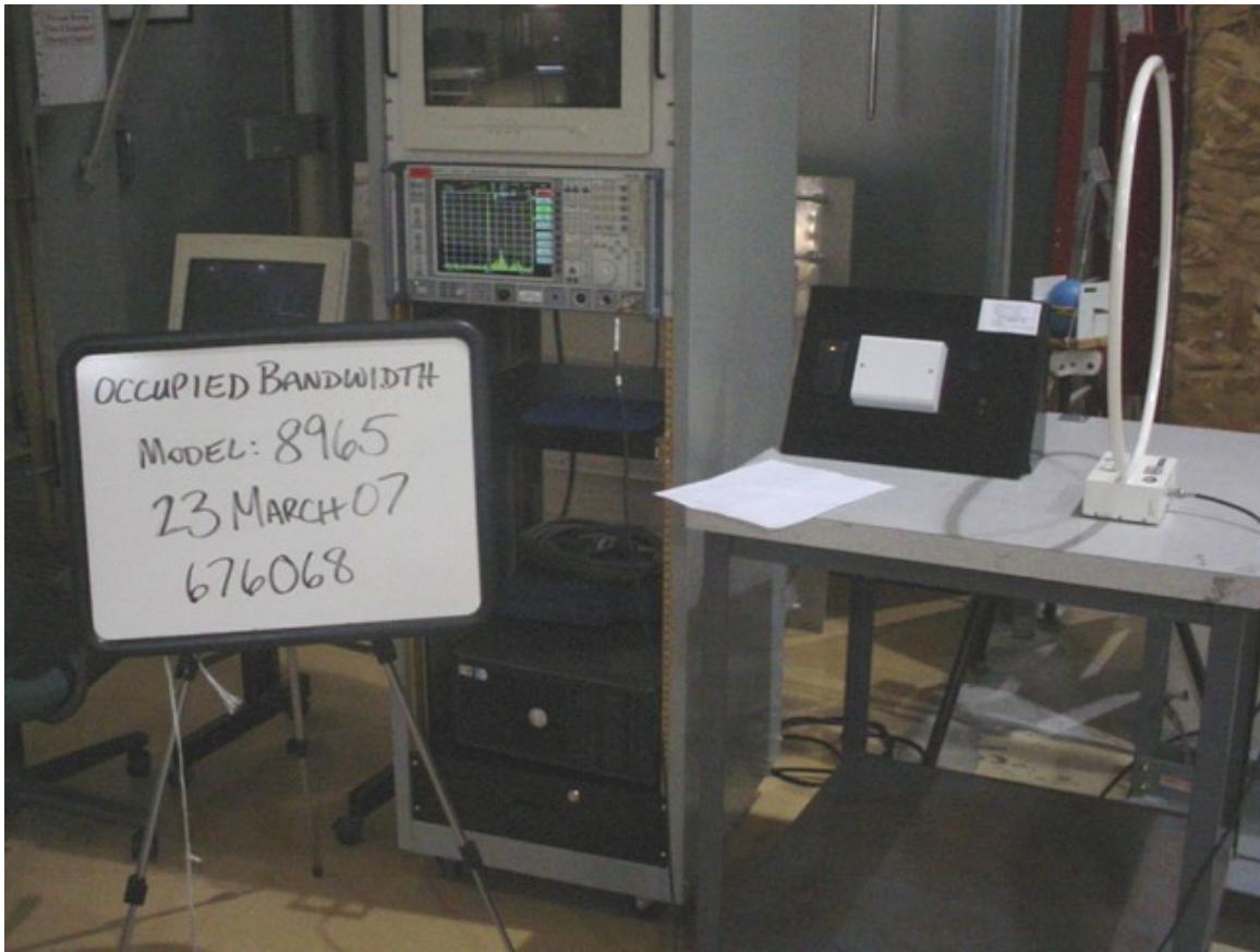
Occupied Bandwidth
