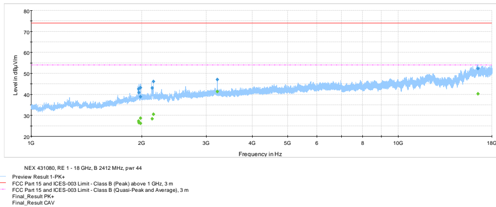
Figure 8.7-12: Radiated spurious emissions 1 – 18 GHz on 802.11b @ 2412 MHz
