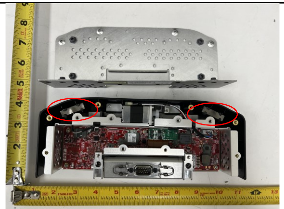
Antenna Position
