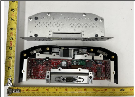
Uncover View
