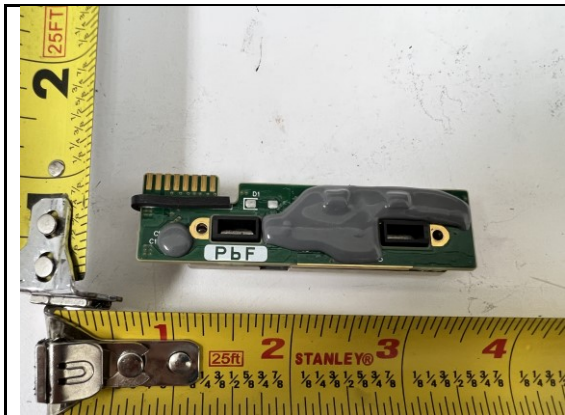
Base connect Board Rear View
