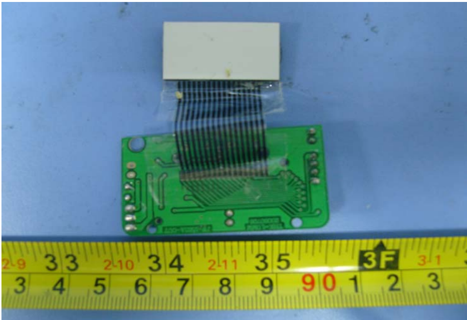
PCB1-Back View
