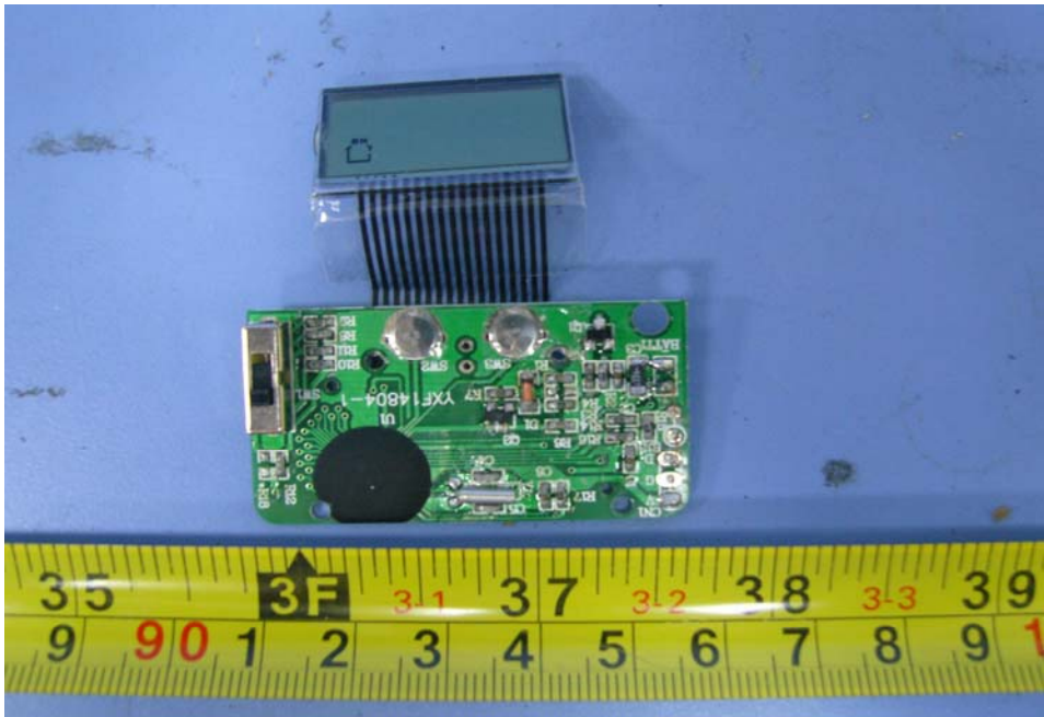
PCB1-Front View
