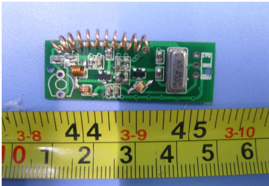
PCB2-Front View
