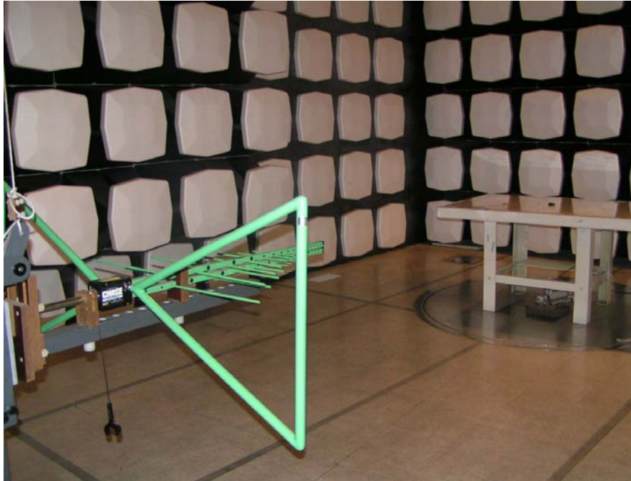
Field Strength Emissions Test Set-up – Lying mode
