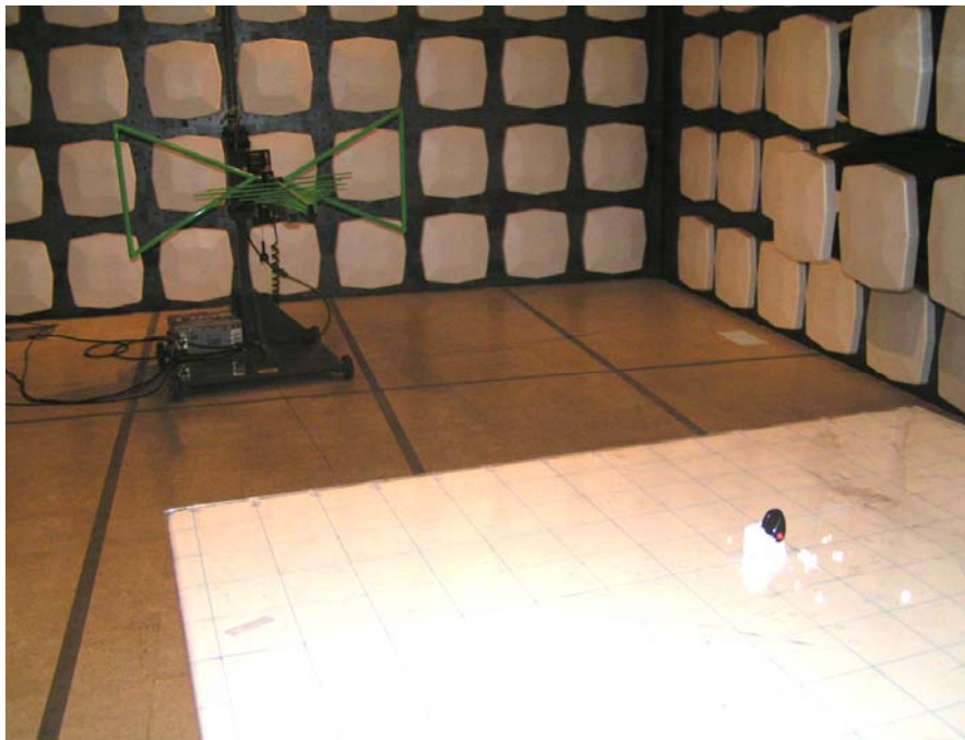
Field Strength Emissions Test Set-up – Side mode
