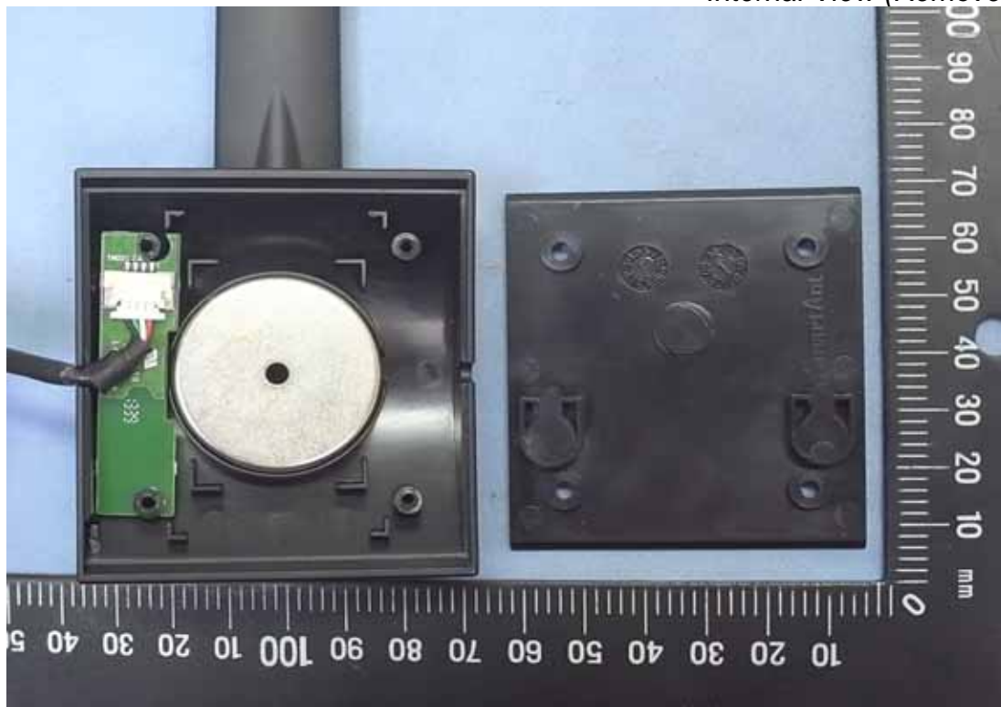
Figure 5 Internal View (Removed Cover)
