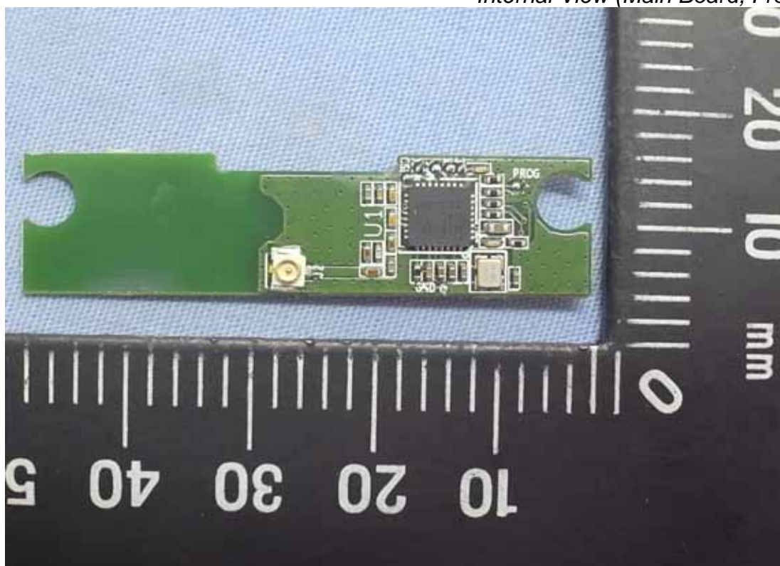
Figure 6 Internal View (Main Board, Front View)
